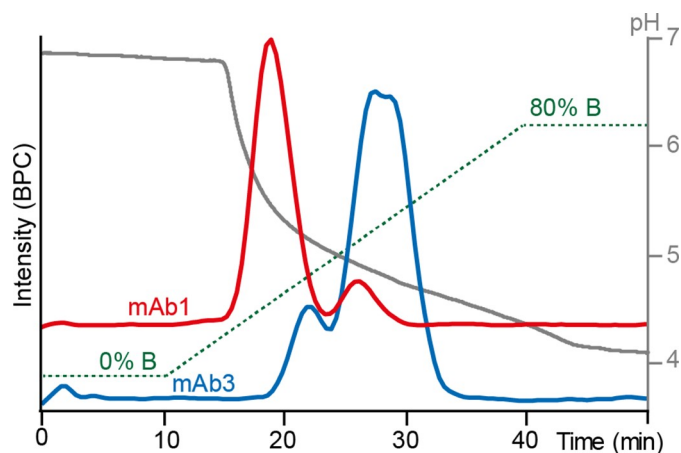
Figure 2. Optimized FcγRIIIb AC-MS gradient. 30 mM ammonium acetate pH 6.8 (solvent A) and 50 mM acetic acid pH 3.0 (solvent B) were used as mobile phases. Base peak chromatograms (BPCs) of mAb1 (red) and mAb3 (blue) are displayed. The gradient (green) and the pH (gray) are displayed as well.
