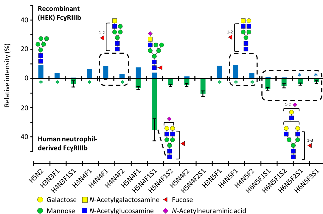
Figure 1. Asn162 glycosylation profiles of FcγRIIIb, comparing recombinant (HEK) and human neutrophil-derived receptor (the latter extracted from Wojcik et al. 23 ). The data was normalized to the sum of all quantified compositions. For recombinant (HEK) FcγRIIIb, these are listed in Table S1. Glycan structures of selected compositions are suggested based on MS/MS experiments and previous findings on HEK cell-derived or human-derived neutrophil FcγRIII glycosylation. 23,27 Asterisks (*) indicate that a glycopeptide was not detected.
