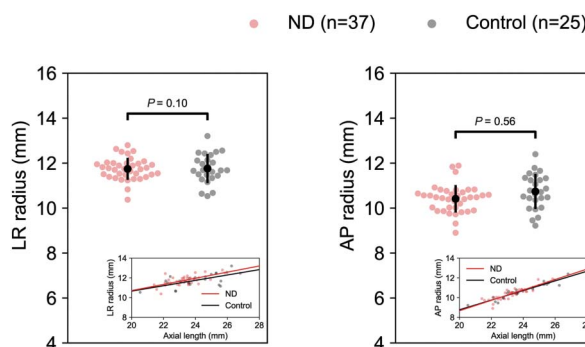
Figure 5. Evaluation of the retinal shape. The shape is quantified by radii in the LR and AP directions for patients with ND (red) and pseudophakic controls (gray) together with the groupwise means (black dots) and SDs (vertical black lines). In addition, the insets show the correlations between these radii and the axial length. All correlations are statistically significant ( P < .01 ), with Pearson r values of \geq 0.65 for the LR radius and \geq 0.88 for the AP radius. When the axial length was taken as a covariate, no statistically significant differences were found between the LR radii ( P = .10 ) or the AP radii ( P = .56 ) of both groups. AP = anterior-posterior; LR = left-right; ND = negative dysphotopsia.
