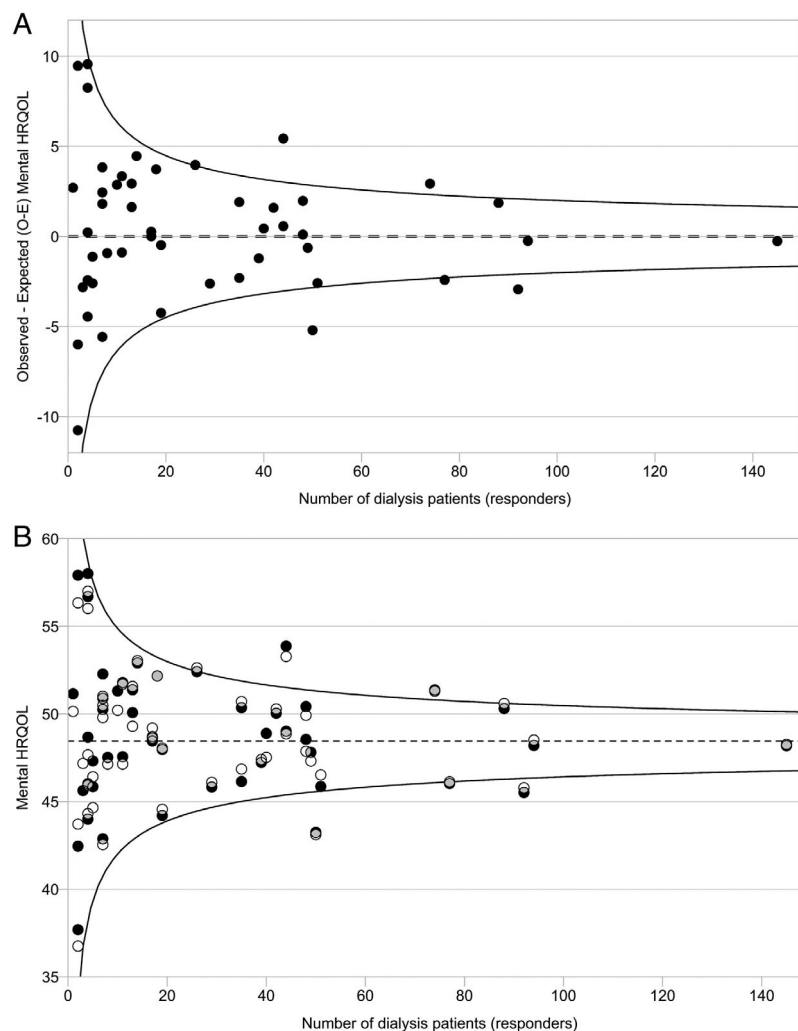
FIGURE 4 A, Funnel plot of comparison between observed and expected scores on mental health-related quality of life (HRQOL) in 48 Dutch dialysis centres. Circles represent the difference between the centres' observed and expected* scores on mental HRQOL of 48 centres that participated in the Dutch registry of patient-reported outcome measures (PROMs) in 2019. The total study population of Dutch dialysis patients is used as a reference standard (dashed line) to compare centres with. The 95% control limits (curved lines) are provided around the reference standard. Four centres exceed the 95% control limits, indicating statistically significant lower (two centres) or higher (two centres) scores on mental HRQOL compared with the reference standard. *Case mix factors included: sex, age, socioeconomic status, primary kidney disease, dialysis modality and time on renal replacement therapy. B, Funnel plot of observed and standardized scores on mental HRQOL in 48 Dutch dialysis centres. Circles represent the mean observed (white circles) and standardized* (black circles) scores on mental HRQOL of 48 centres that participated in the Dutch registry of PROMs in 2019. Overlapping part of circles is depicted grey. The overall mean score on mental HRQOL of all Dutch dialysis patients (dashed line) is used as reference standard to compare centres with. The 95% control limits (curved lines) are provided around the reference standard. The standardized scores of four centres exceed the 95% control limits, indicating statistically significant lower (two centres) or higher (two centres) scores on mental HRQOL compared with the reference standard. *Standardized score = observed score – expected score + reference score. The following case mix factors were included to calculate the expected scores: sex, age, socioeconomic status, primary kidney disease, dialysis modality and time on renal replacement therapy
