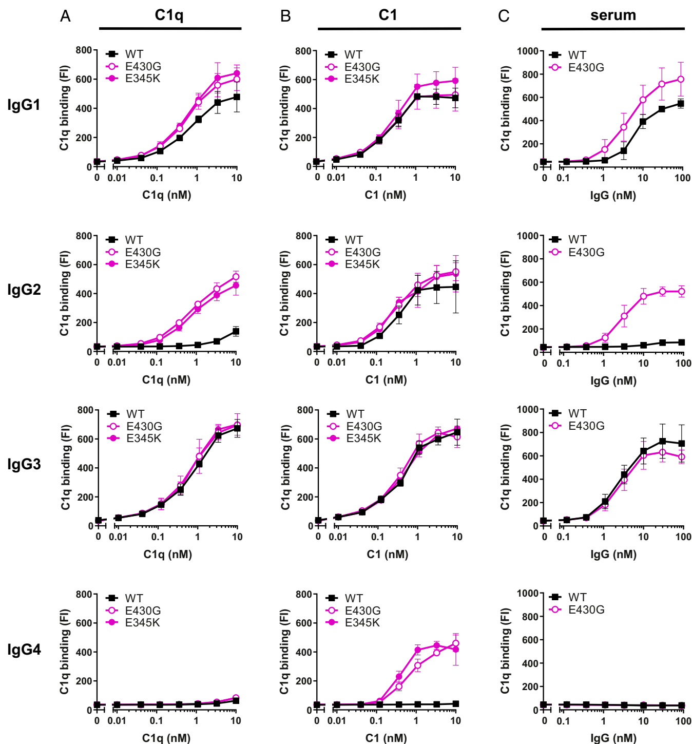
Fig. 5. Enhanced IgG oligomerization stabilizes C1q-IgG interactions. (A and B) Binding of purified C1q (A) or C1 (B) to DNP beads (1 \mu g/mL DNP) labeled with 20 nM anti-DNP IgG, either wild-type or containing hexamer-enhancing mutations E430G or E345K. (C) Detection of C1q on DNP-beads (1 \mu g/mL DNP) after incubation with 1% \Delta IgG \Delta IgM serum supplemented with wild-type or mutated (E430G) anti-DNP IgG. (A–C) C1q was detected by flow cytometry. The data represent geometric mean \pm SD of three independent experiments.
