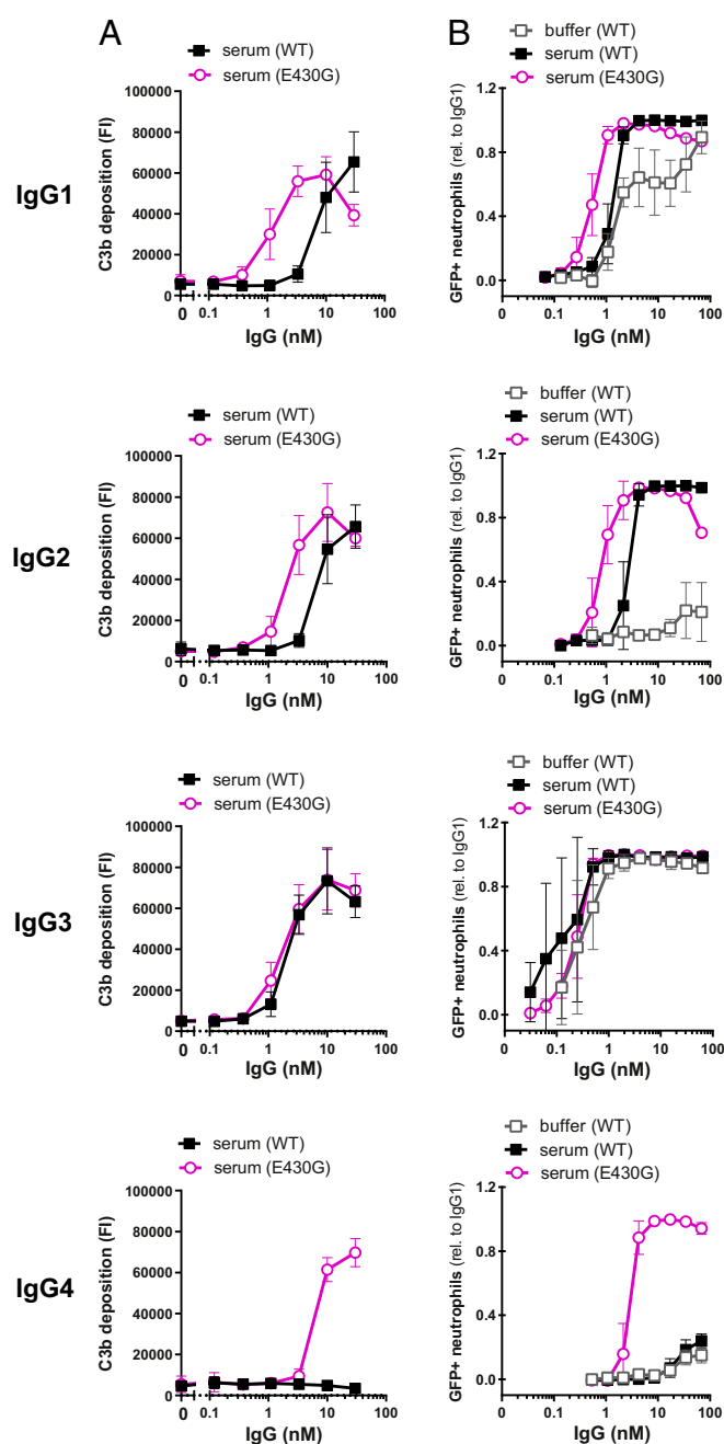
Fig. 6. Introduction of hexamer-enhancing mutation E430G in anti-WTA can enhance complement-dependent phagocytosis of S. aureus . (A) C3b deposition on S. aureus Wood46 after incubation of bacteria in 5% \Delta IgG \Delta IgM serum supplemented with anti-WTA IgG (wild-type or E430G mutant). The data represent mean \pm SD of three independent experiments. (B) Phagocytosis in the absence and presence of complement. Phagocytosis of fluorescently labeled S. aureus Wood46 in either RPMI buffer or 1% \Delta IgG \Delta IgM serum supplemented with anti-WTA IgG (wild-type or E430G mutant) and human neutrophils. Bacterial uptake was quantified by flow cytometry and displayed as the number of GFP-positive neutrophils relative to IgG1 wild type. The data represent relative mean \pm SD of three independent experiments. Phagocytosis data shown for wild-type IgG2 (buffer and serum condition) are identical to the data shown in Fig. 1C.
