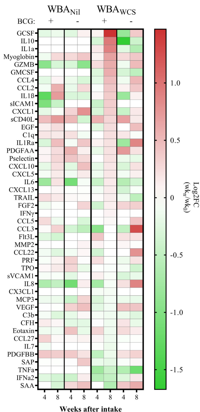
Fig. 3. Longitudinal immune profiling in BCG-vaccinated household contacts of leprosy patients. Forty-six CCGFs were determined in WBA from household contacts (HC) receiving BCG ( n = 16 ) and HC of leprosy patients without an intervention ( n = 16 ). Blood was collected at intake (just before vaccination in the BCG group) and 4 and 8 weeks after intake. Levels of the 46 CCGFs were measured in unstimulated whole blood assay supernatant and in response to M. leprae whole cell sonicate (WCS). All samples were tested in the same experiment and randomly distributed over multiple 96-wells plates. The heatmap displays the median Log2FC of the concentration level at the respective weeks ( wk_n ) compared to the level at intake ( wk_0 ). An increased level over time compared to wk_0 is indicated in red and a decreased level in green. (For interpretation of the references to colour in this figure legend, the reader is referred to the web version of this article.)
