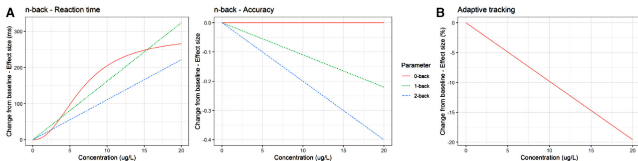
Figure 4. Visualization of the typical concentration-effect relationships for the n-back (A) and the adaptive tracking (B) tasks.
