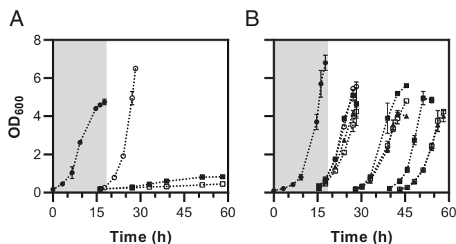
Fig. 1. Anaerobic growth of S. cerevisiae CEN.PK113-7D and Sch. japonicus CBS5679 with different ergosterol and UFA (Tween 80) supplementation in a dark anaerobic chamber. Anaerobic precultures on SMPD on 50 \text{ g} \cdot \text{L}^{-1} glucose (closed circles, gray shading) were grown until the end of the exponential phase. (A) After the anaerobic preculture, S. cerevisiae was transferred to SMPD ( 20 \text{ g} \cdot \text{L}^{-1} glucose) supplemented with either Tween 80 and ergosterol (open circles), Tween 80 only (closed squares), or neither Tween 80 nor ergosterol (open squares). (B) Sch. japonicus was grown on the same media as S. cerevisiae and additionally on medium containing ergosterol but not Tween 80 (closed triangles). Sch. japonicus cultures supplemented with only Tween 80, only ergosterol, and those without supplements were serially transferred to fresh media with the same composition in the anaerobic chamber. Data are represented as average \pm SEM of measurements on independent duplicate cultures for each combination of yeast strain and medium composition.
