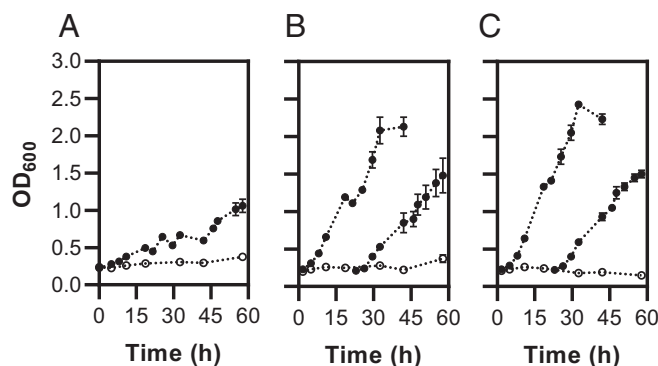
Fig. 6. Anaerobic growth of S. cerevisiae strains in sterol-free media. S. cerevisiae cultures were inoculated from an anaerobic preculture on SMPD (50 g · L -1 glucose) to fresh SMPD (20 g · L -1 glucose), either supplemented with Tween 80 (closed circles), or lacking UFAs and sterols (open circles). (A) Reference strain CEN.PK113-7D. (B) S. cerevisiae strain IMX2616 ( sga1Δ::Sjshc1 ). (C) S. cerevisiae strain IMX2629 ( sga1Δ::Sjshc1 X-2::Maths ). Cultures supplemented with Tween 80 represented in panels (B) and (C) were transferred to fresh medium of the same composition (closed circles) during exponential phase. Data are represented as average ± SEM of measurements on independent duplicate cultures for each yeast strain.
