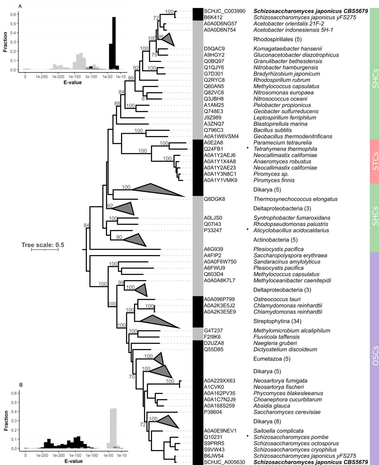
Fig. 5. Maximum-likelihood phylogenetic tree of selected triterpenoid cyclases. The colored bar indicates different types of cyclases: green, SHCs; red, STCs; and purple, OSCs. Sequences were obtained from a systematic homology search using the characterized cyclases marked with an asterisk (A. alicyclobacillus AaShc, P33247, SHC; T. thermophila , TtThc1, Q24FB1, STC; Schizosaccharomyces pombe SpErg7, Q10231, OSC) as queries. Eukaryotic and bacterial sequences are indicated by black and gray bars, respectively. Clades were collapsed when having three or more members from the same taxonomic division (third level below Bacteria or Eukaryota according to NCBI taxonomy) with the exception of Neocallimastogomycetes and Schizosaccharomycetes. A total of 100 bootstrap replicates were performed, values above 70 are shown on the corresponding branches. All sequences and the final tree are provided in Datasets S3 and S4 , respectively. The tree was midrooted, visualized, and made available in iTOL ( https://itol.embl.de/tree/19319025314539181623851833 ). (A) Distribution of HMMER E-values obtained with Sch. japonicus SHC (SCHJC_C003990) as query against a bacterial sequence database (gray bars) and a eukaryotic database (black bars). (B) Distribution of HMMER E-values obtained with Sch. japonicus OSC (SCHJC_A005630) as query against a bacterial sequence database (gray bars) and a eukaryotic database (black bars).
