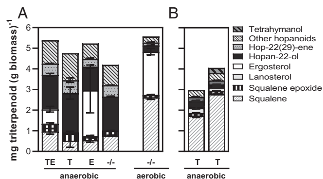
Fig. 4. Quantification of triterpenoids in yeast biomass. (A) Triterpenoid content of cultures of Sch. japonicus CBS5679 grown in SMPD with 20 g \cdot L ^{-1} glucose. Under anaerobic conditions, cultures were supplemented with Tween 80 and ergosterol (TE), only ergosterol (E), only Tween 80 (T), or neither of these supplements (–/–). Data are shown for the first anaerobic culture following the anaerobic pre-culture. Aerobic cultures of Sch. japonicus were grown in SMPD without supplements (–/–). (B) Triterpenoid composition of anaerobic cultures of S. cerevisiae IMX2616 ( sga1 \Delta ::Sjshc1 ; Left) and IMX2629 ( sga1 \Delta ::Sjshc1 X-2::Maths ; Right) grown in SMPD with 20 g \cdot L ^{-1} glucose and Tween 80 (T) supplementation. Data are represented as average \pm SEM of data from two independent duplicate cultures for each cultivation condition. Detailed information on data presented in this figure and additional anaerobic transfers are provided in Dataset S1.
