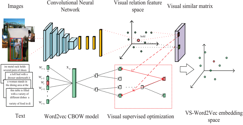
Figure 2.1: VS-Word2Vec Framework.
