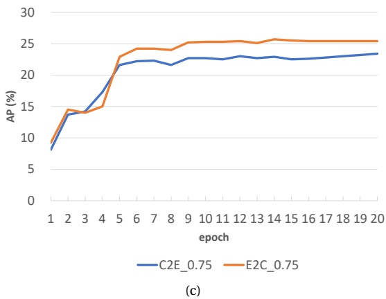
Figure 3.8: Results of LICN-E2C and LICN-C2E on the FG-sCOCO validation set for different training epochs. (a) Mean AP of 0.50:0.95 in steps of 0.05, (b) AP of 0.5, and (c) AP of 0.75.
