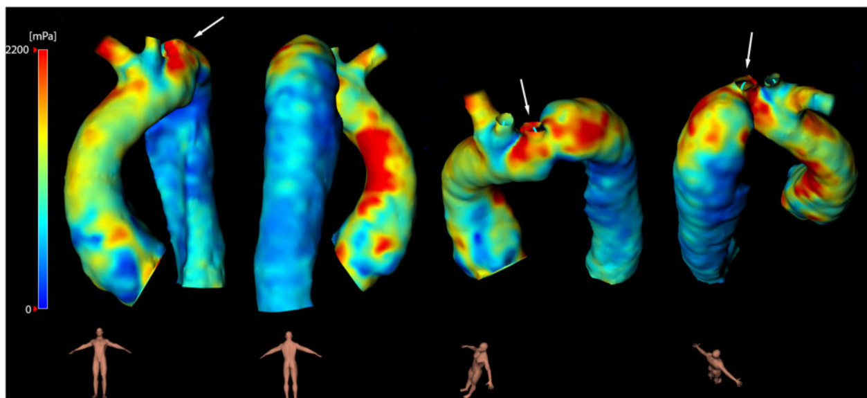
Figure 2 Type B dissection ascending, arch and false lumen (true lumen not included) wall shear stress magnitude maps derived from 4D flow magnetic resonance imaging. The arrow indicates the location of high wall shear stress surrounding the left subclavian artery. 4D flow parameters were analysed using CAAS MR Solutions 5.2; Pie Medical Imaging, Maastricht, The Netherlands. Colour scale from blue (representing low wall shear stress) to red (representing higher \geq 2200 mPa wall shear stress). Colour scale is provided on the left side of the image.
