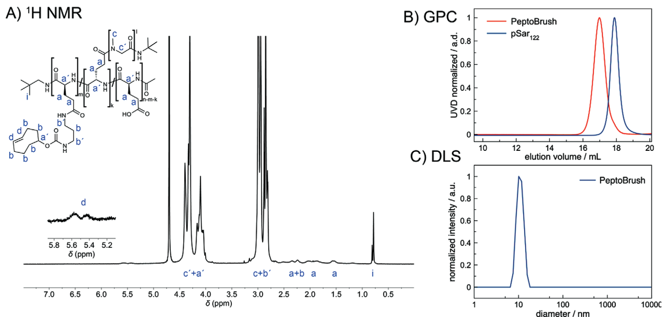
Figure 2. Characterization of the TCO-containing PeptoBrushes 1: A) ^1\text{H} -NMR of in \text{D}_2\text{O} . B) GPC characterization of pSar side chains and final graft copolymers in hexafluoroisopropanol (HFIP), C) DLS in PBS buffer.
