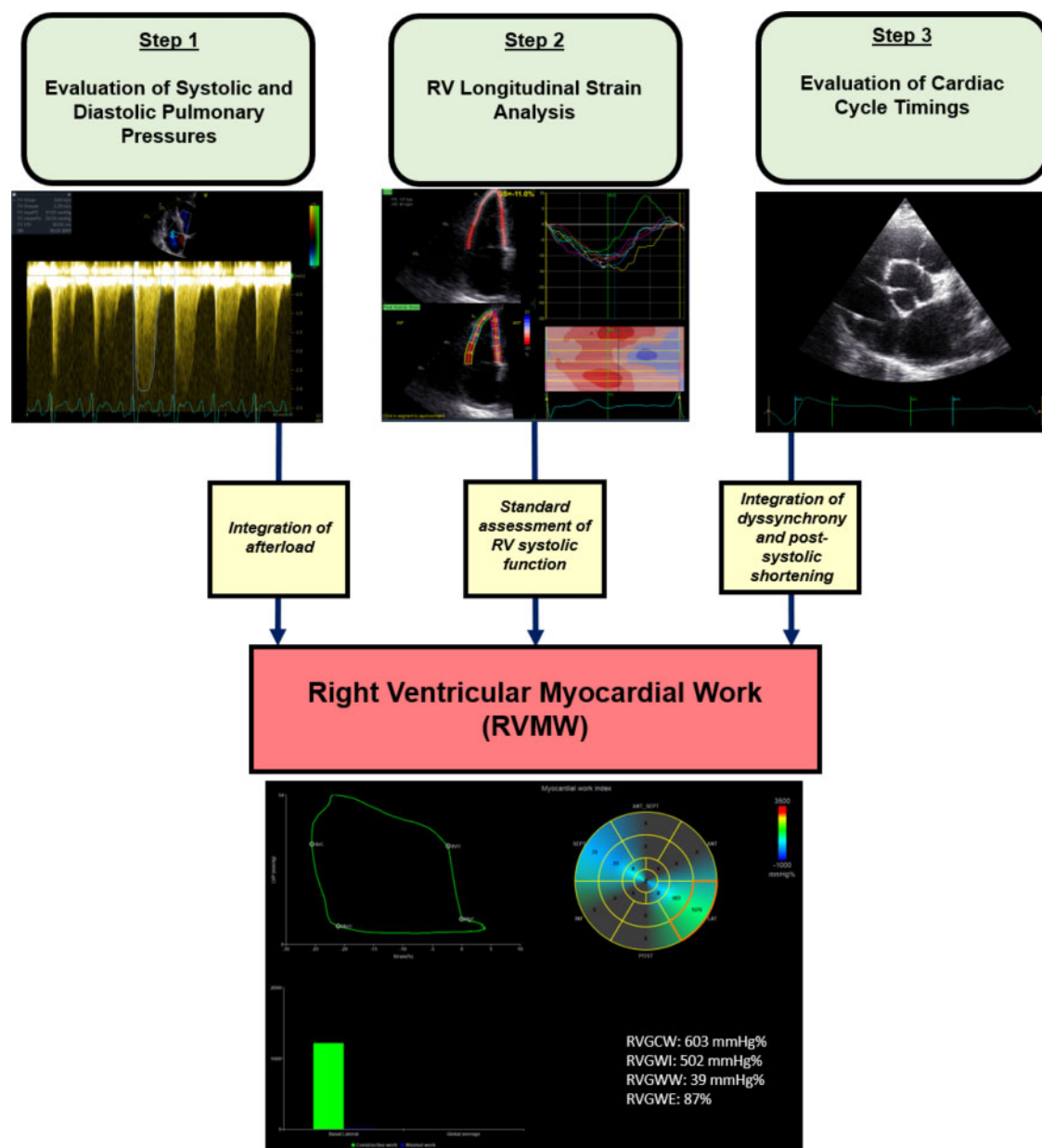
Figure 2 Method for the calculation of RVMW. RVMW provides an integrative analysis of RV function, incorporating speckle tracking echocardiography-derived RV strain, pulmonary pressures, and cardiac cycle timings. Cardiac cycle timings are determined by pulmonic and tricuspid valve opening and closure events, identified through either direct visualization of two-dimensional images or by pulsed-wave Doppler interrogation. Integration of event timings allows for the quantitative evaluation of RV dyssynchrony and post-systolic contraction. Indices of RVMW are calculated based on non-invasively derived pressure-strain loops for the right ventricle. RV, right ventricular; RVGCW, right ventricular global constructive work; RVGWE, right ventricular global work efficiency; RVGWI, right ventricular global work index; RVGWW, Right ventricular global wasted work; RVMW, right ventricular myocardial work.
