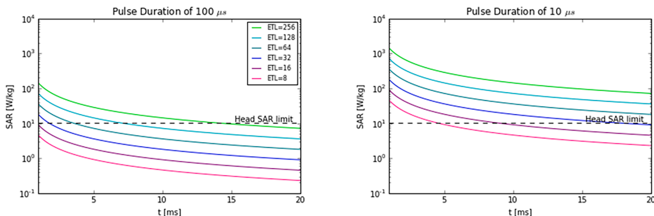
Fig. 10. Calculated specific absorption rate (SAR) as a function of the inter-pulse time ( t ) for a TSE sequence with different echo train lengths (ETLs). The pulse durations are (left) 100 \mu s and (right) 10 \mu s. The head SAR limit (10 W/kg) (24) is shown by the dashed line.
