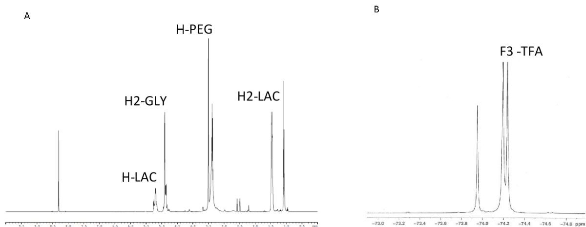
Figure 2. NMR characterization of functional copolymers. (A) ^1\text{H} -NMR spectrum of PLGA-PEG-TFA in DMSO. (B) ^{19}\text{F} -NMR spectrum of PLGA-PEG-TFA in \text{D}_2\text{O} .
