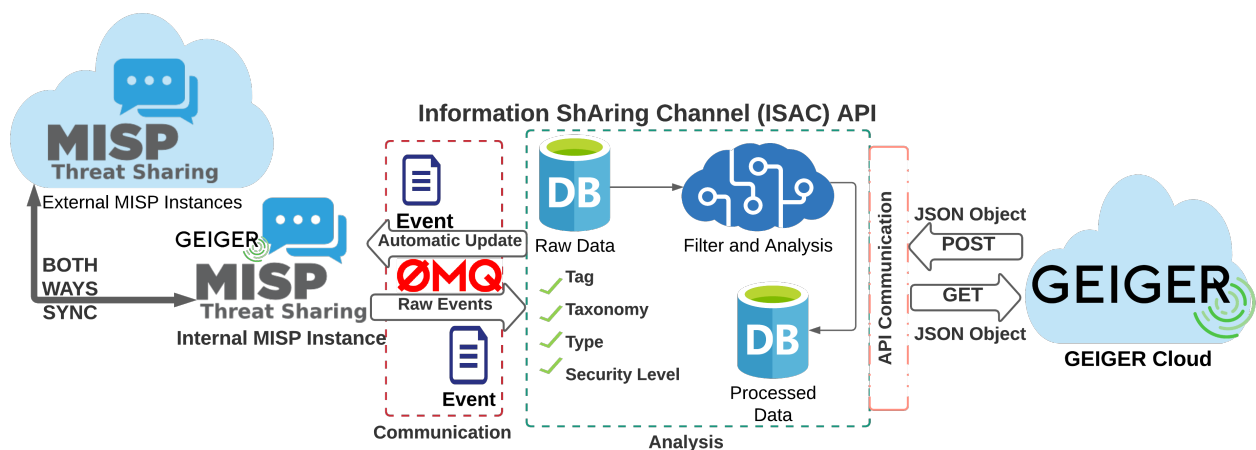
Figure 3. Incoming MISP data processed by the GEIGER information sharing channel and stored in the GEIGER cloud storage.
