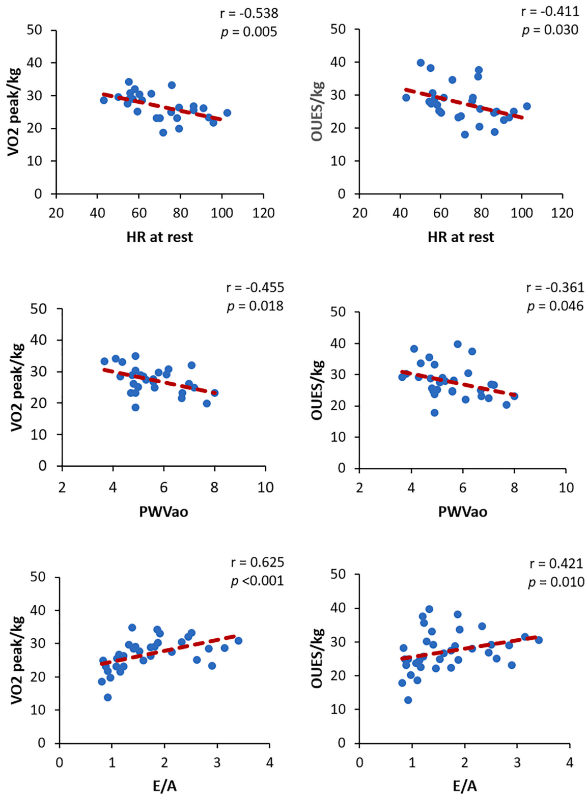
Fig. 1. Correlation between VO 2 peak or OUES and HR, PWVao and E/A.
