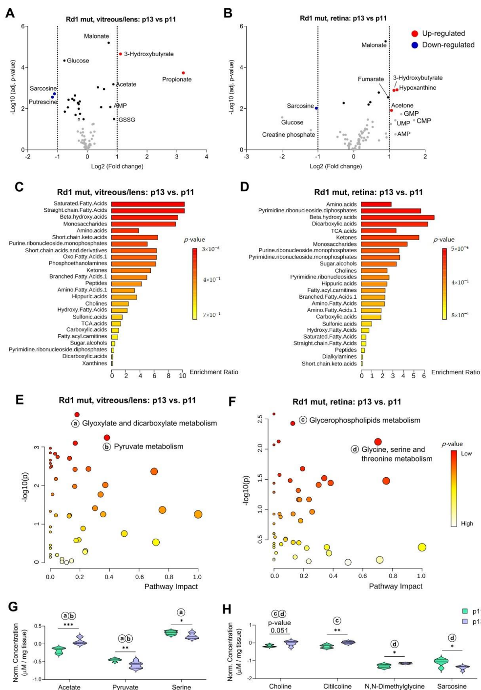
Figure 4. Photoreceptor degeneration affects the metabolite composition of vitreous/lens and retina across time. ( A,B ) Volcano plots with the differences between time-point p13 and p11 of metabolites concentration in the vitreous/lens ( A ) and the retina ( B ) of Rd1 mutant mice. ( C,D ) Quantitative metabolite set enrichment analysis showing the metabolite classes enriched in vitreous/lens ( C ) and retina ( D ) between the two time-points. ( E,F ) Pathway analysis with the significance of the time-point comparison in the vitreous/lens ( E ) and retina ( F ) in relation to the topology (impact). Selected pathways with a high significance are indicated (small letters). ( G,H ) Violin plots with summary quantification data of metabolites with a high significance within the indicated pathways in subfigures ( E,F ) in the vitreous/lens ( G ) and retina ( H ). The concentrations are showed at both time-points. The letters indicate the pathway in subfigures ( E,F ) in which the metabolites are found. Vitreous/lens: n = 6 (p11), n = 7 (p13). Retina: n = 5 (p11), n = 6 (p13). Multiple unpaired t test with Holm–Šidák correction for multiple comparisons. * p < 0.05 , ** p < 0.01 , *** p < 0.001 .
