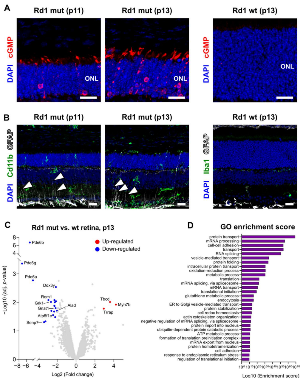
Figure 1. Retinal degeneration in the Rd1 mutant mouse. (A) Maximum intensity projection of confocal images showing immunolocalization of cGMP (red) in the outer nuclear layer (ONL) in the Rd1 mutant mouse at p11 and p13 and in the Rd1 wt control at p13. (B) Reactivity and distribution of glial cells across different retina layers. Arrowheads indicate the processes of Müller glia cells with a positive GFAP signal. (C) Volcano plot of protein expression ratios between Rd1 mutant and Rd1 wt at p13. Dots in blue or red indicate proteins that are significantly down- or up-regulated, respectively. (D) Gene Ontology analysis performed on all proteins and showing the 30 terms with the highest enrichment score. Rd1 wt: n = 4 ; Rd1 mutant: n = 4 . Scale bars: 20 \mu m.
