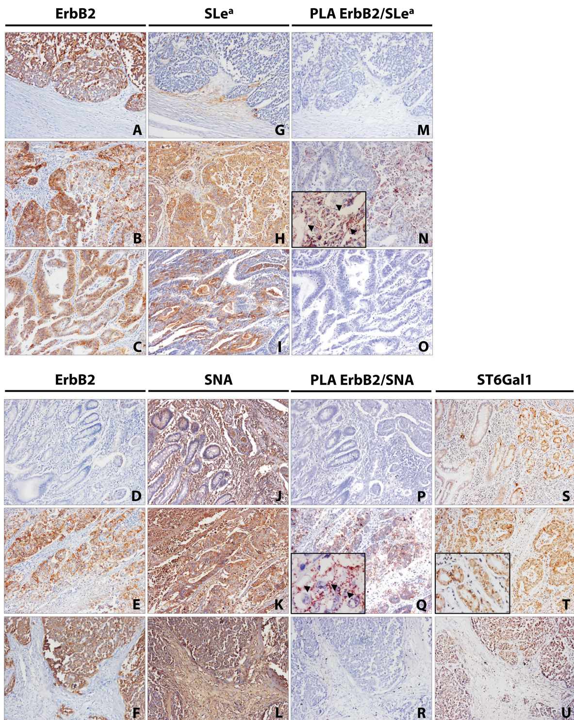
Fig. 1 Expression of ErbB2 sialylated glycoforms in intestinal-type gastric carcinoma. Representative individual (immuno)histochemical detection of: ErbB2 (A–F), sialyl Lewis a (SLe a ) (G–I), and Sambucus nigra agglutinin (SNA) ( \alpha 2,6-linked sialic acid ( \alpha 2,6NeuAc)) (J–L) in gastric carcinoma tissue sections; Parallel in situ brightfield Proximity
