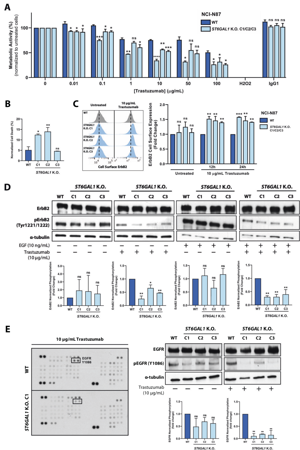
Fig. 6 ST6GAL1 K.O. sensitizes ErbB2-positive gastric cancer cells to trastuzumab-induced cytotoxicity. A Resazurin assay for the measurement of the metabolic activity of NCI-N87 WT and ST6GAL1 K.O. ErbB2-positive gastric cancer (GC) cells following the treatment with increasing doses of trastuzumab; H 2 O 2 —positive control; IgG1—trastuzumab isotype control; B Assessment of trastuzumab-induced cell death through the annexin V/propidium iodide (PI) staining of WT and ST6GAL1 K.O. cells treated with 10 µg/mL trastuzumab for 120 h; C Quantification of ErbB2 cell surface expression by trastuzumab-binding in WT and ST6GAL1 K.O. cells treated with 10 µg/mL trastuzumab for 12 and 24 h; D Western blot analysis and \alpha -tubulin-normalized quantification of ErbB2 intracytoplasmic phosphorylation in WT and ST6GAL1 K.O. cells treated with 10 µg/mL trastuzumab for 120 h and stimulated with 10 ng/mL EGF; E Analysis of the phosphorylation status of 43 human kinases in NCI-N87 WT and ST6GAL1 K.O. cells treated with 10 µg/mL trastuzumab for 120 h; Western blot analysis and \alpha -tubulin-normalized quantification of EGFR intracytoplasmic phosphorylation for array target validation in NCI-N87 WT and ST6GAL1 K.O. cells treated with 10 µg/mL trastuzumab for 120 h; Comparisons were made using one-way ANOVA analysis of variance ( n = 3 ; mean \pm SD; * p < 0.05 ; ** p < 0.01 ; *** p < 0.001 ; n.s. nonsignificant, C1 clone 1, C2 clone 2, C3 clone 3).
