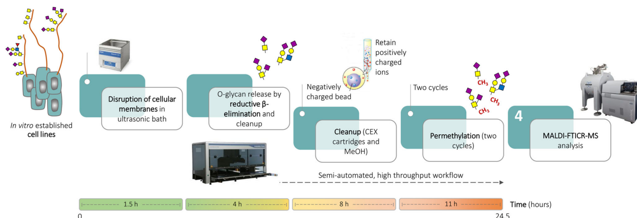
Fig. 1 Workflow for semi-automated, high throughput reductive \beta -elimination, coupled to ultrahigh resolution MALDI-FT-ICR MS for O-glycosylation analysis of in vitro established cell lines
