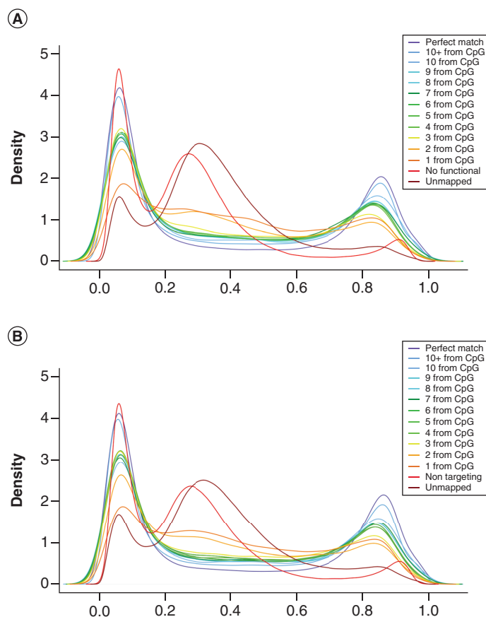
Figure 3. Density distribution of beta-values for mapped and unmapped Infinium 450K CpG probes. Mapped probes for Chlorocebus sabaeus (A) and Macaca mulatta (B) are classified into categories representing probes with a perfect match and according to the mismatch position localized from 1 bp to 10 bp or more from the CpG dinucleotide. Probes containing a mismatch localized at 1 or 2 bp (dark orange and orange) do no longer show the expected beta-value density distribution compared with the other mapped probes (yellow, greens, blues and purple). Nontargeting probes (red) and unmapped probes (dark red) have an aberrant beta-value distribution. For reasons of clarity only the average density curve derived from 21 C. sabaeus and 25 M. mulatta samples is shown.
