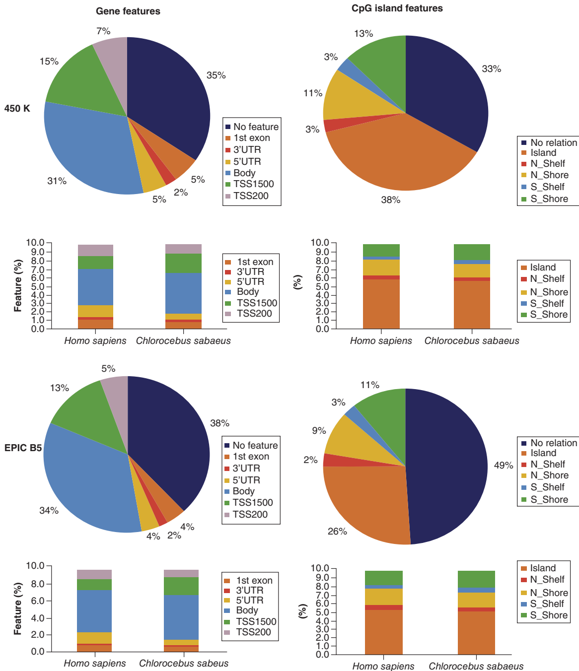
Figure 6. Piecharts represent the distribution of human-designed Chlorocebus sabaeus -valid CpG probes on the Infinium 450K and EPIC BeadChips, as annotated for the Chlorocebus sabaeus genome (Ensembl ChISab1.1 version 101). We defined 162,053 C. sabaeus -valid probes for Infinium 450K and 255,227 for Infinium EPIC, representing 171,608 and 267,827 gene feature annotations in total for Infinium 450K and Infinium EPIC, respectively. Note that one probe can be attributed to different transcripts and thus gene features, whereas one probe is attributed to only one island feature. The stacked barplots show the gene feature and CpG island annotation in comparison to the same probes annotated to the human arrays, as given in the BeadChip manifest files.
