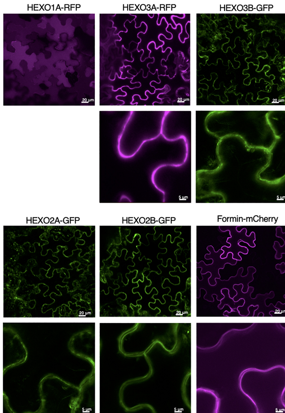
FIGURE 3 | Subcellular localization of Nicotiana benthamiana HEXOs. GFP- or RFP-tagged HEXOs or formin-mCherry (used as plasma membrane marker) were transiently expressed in N. benthamiana leaves. Whole mount confocal microscopy pictures were taken at 3 days post infiltration. For each construct overview pictures are given (scale bar of 20 \mu m) and a picture at higher magnification underneath (scale bar 5 \mu m).
