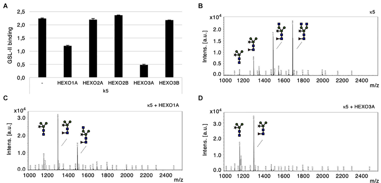
FIGURE 4 | Cleavage of terminal GlcNAc residues by N. benthamiana HEXOs. Kappa-5 was co-expressed with p19 and different HEXO genes in wild-type plants. After isolation of the apoplast fluid (at 6 dpi) the glycan composition of kappa-5 was analyzed. (A) Griffonia simplicifolia lectin II (GSL-II) binding assay for detection of terminal GlcNAc. Lectin binding is measured as absorbance at 450 nm. (B–D) Kappa-5 was purified from the apoplast fluid and the N-glycan composition was analyzed by MALDI-TOF-MS. MS profiles are given for N-glycans of wild-type kappa-5 (B) or upon co-expression of HEXO1A (C) or HEXO3A (D) . m/z refers to mass-to-charge ratio.
