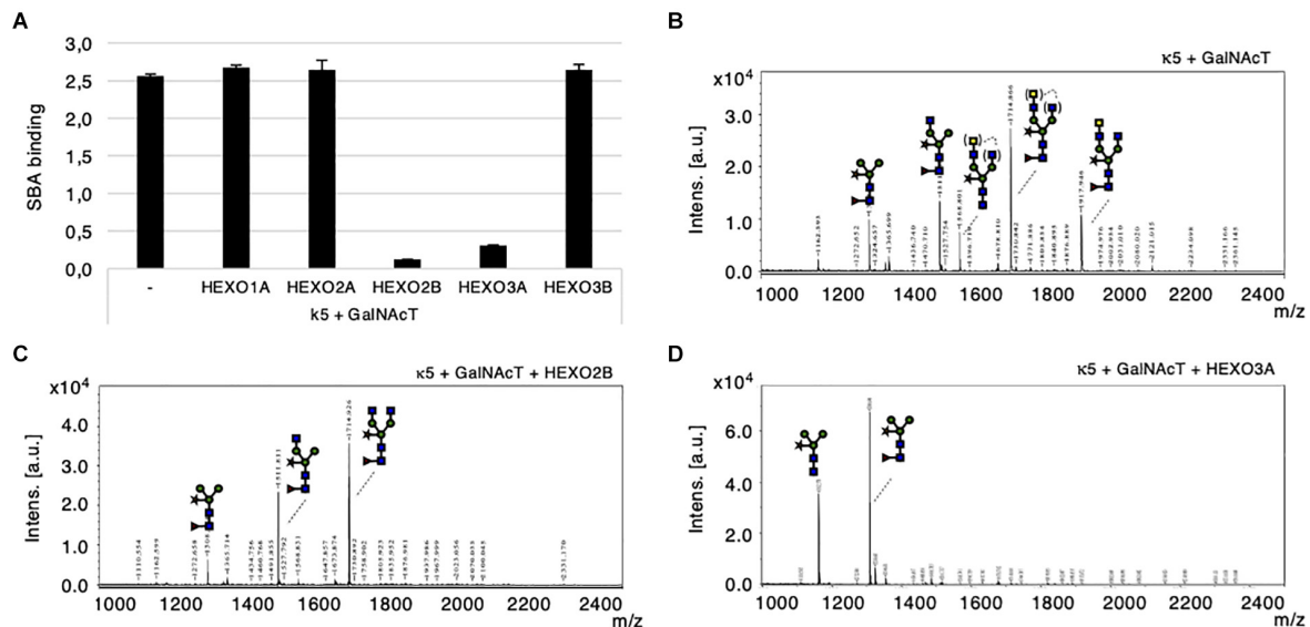
FIGURE 5 | Cleavage of engineered LDN motifs by N. benthamiana HEXOs. Kappa-5 was co-expressed with p19, CeGalNAcT and different HEXO genes in wild-type plants. After isolation of the apoplast fluid (at 6 dpi) the presence of the LDN motif on kappa-5 N-glycans was analyzed. (A) Soybean agglutinin (SBA) binding assay for detection of terminal GalNAc. Lectin binding is measured as absorbance at 450 nm. (B–D) Kappa-5 was purified from the apoplast fluid and the N-glycan composition was analyzed by MALDI-TOF-MS. MS profiles are given for N-glycans of kappa-5 upon co-expression of GalNAcT only (B) , or combined with co-expression of HEXO2B (C) , or HEXO3A (D) . When a MS peak represents multiple N-glycan structures of identical mass, the possible positions of these sugar residues on the N-glycan are indicated between brackets. m/z refers to mass-to-charge ratio.
