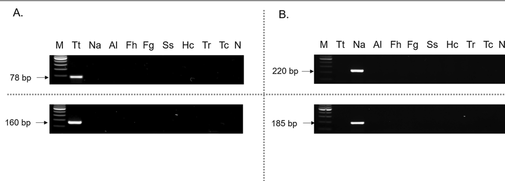
Fig. 3 Specificity of the pyrosequencing assays for T. trichiura and N. americanus . Specificity assessment performed with the primers for A T. trichiura and B N. americanus is shown. Upper figures show the PCR reaction using the primers for detecting the SNP at codon 167; down figures refer to the primers for the SNPs at codons 198 and 200. The amplicon size is shown in the right position of the gel and it is expressed in base pair (bp). Lane M, 100 bp DNA ladder; lanes Tt, Na, Al, Fh, Fg, Ss, Hc, Tr, Tc, T. trichiura , N. americanus , A. lumbricoides , Fasciola hepatica , Fasciola gigantica , Strongyloides stercoralis , Haemonchus contortus , Trichostrongylus spp. and Teladorsagia circumcincta DNA samples, respectively; lane N, negative control (no DNA template)
