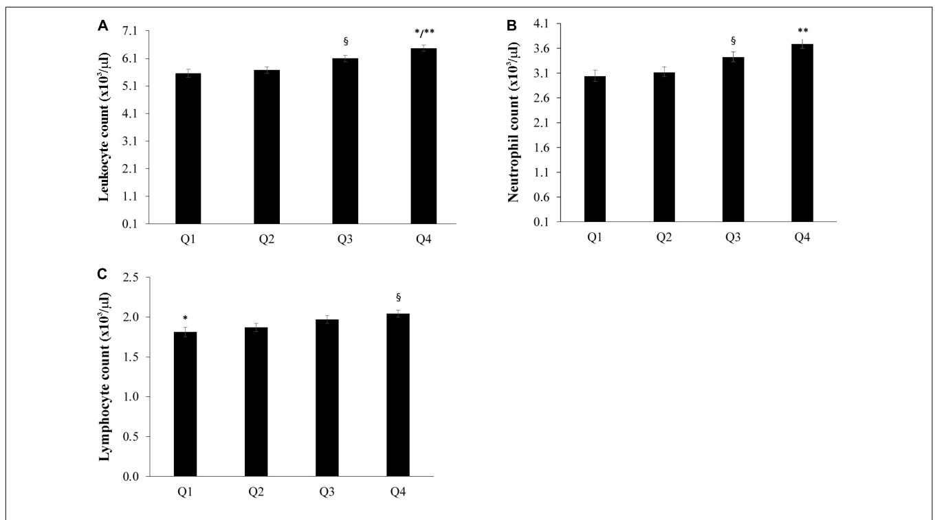
FIGURE 3 | Relationship between bacterial DNA quartiles and (A) whole blood leukocytes, (B) neutrophil count, and (C) lymphocyte count. The fourth quartile (Q4) of bacterial DNA levels displayed the highest levels of leukocytes, lymphocytes and neutrophils than the other quartiles. ANCOVA analysis correcting for age, countries, gender, BMI, smoke habits and Self-rated health status was applied; data are reported from the model adjusted mean \pm Standard Error of the Mean (SEM); ** p < 0.001 as compared to Q1 and Q2; § p < 0.05 as compared to Q1 and Q2; * p < 0.05 as compared to Q3.
