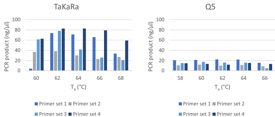
Figure 2. Varying T_a and the respective amount of PCR product, using commercial human DNA (100 ng) with four different primer sets, split for the TaKaRa and Q5 polymerase. T_a =primer annealing temperature; PCR=polymerase chain reaction.
