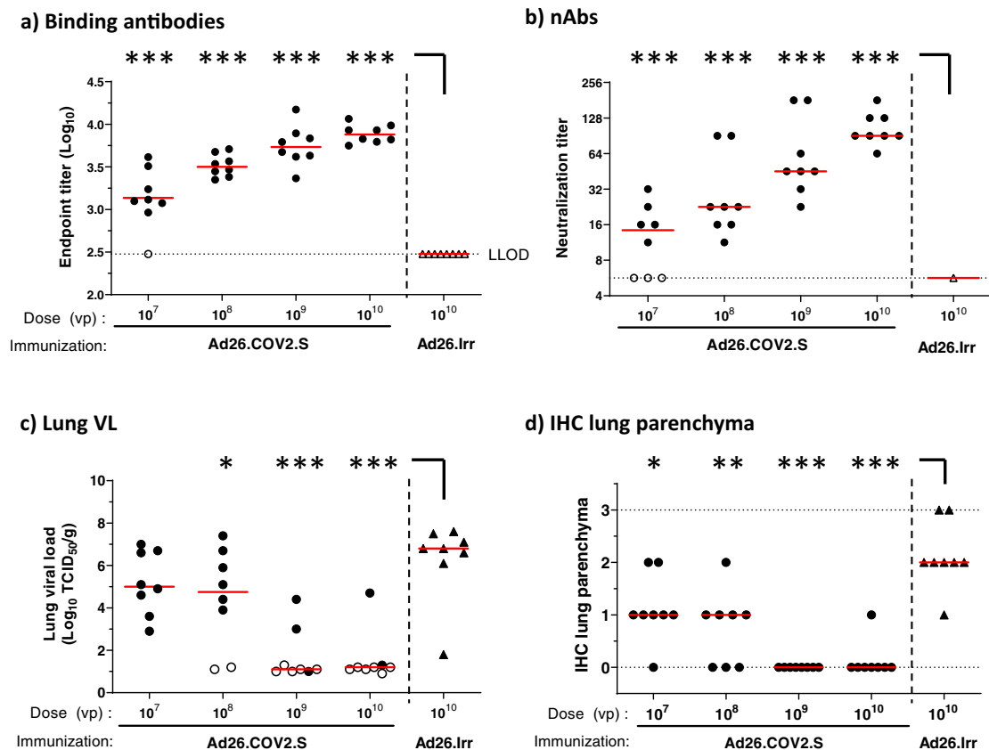
Fig. 4 Dose responsiveness of Ad26.COV2.S on immunogenicity and lung viral load in hamsters. Syrian hamsters were intramuscularly immunized with 10^7 , 10^8 , 10^9 , or 10^{10} VP of Ad26.COV2.S ( N = 8 per group), or 10^{10} VP Ad26.Irr (an Ad26 vector not encoding any SARS-CoV-2 antigens, N = 8 ). Four weeks after one immunization, SARS-CoV-2 Spike protein-specific antibody-binding titers as measured by ELISA (a) and SARS-CoV-2-neutralizing antibodies as measured by wtVNA (b) were determined. The median antibody responses per group is indicated with a horizontal line. Dotted lines indicate the LLOD. Animals with a response at or below the LLOD were put on LLOD and are shown as open symbols. Hamsters received intranasal inoculation with 10^2 TCID 50 SARS-CoV-2 strain BetaCoV/Munich/BavPat1/2020 4 weeks post immunization (week 4). Right lung tissue was isolated 4 days after inoculation for virological analysis and immunohistochemistry. c Lung viral load was determined by TCID 50 assay on Vero E6 cells. The median viral load per group is indicated with a horizontal line. LLOD was calculated per animal, and animals with a response at or below the LLOD are shown as open symbols. d The presence of SARS-CoV-2 NP was determined by immunohistochemical staining. Comparisons were performed between the Ad26.COV2.S dose level groups, with the Ad26.Irr group by Mann–Whitney U test. Statistical differences indicated by asterisks: * p < 0.05 ; ** p < 0.01 ; *** p < 0.001 . Ad26.Irr Ad26 vector not encoding any SARS-CoV-2 antigens, LLOD lower limit of detection, N number of animals, TCID 50 /g 50% tissue culture infective dose per gram tissue, VP virus particles, NP nucleocapsid protein, wtVNA wild-type virus neutralization assay.
