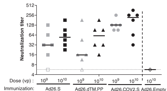
Fig. 2 SARS-CoV-2 neutralizing antibody response elicited by one- and two-dose Ad26.COVS vaccine regimes in Syrian hamsters. a Syrian hamsters were immunized with either 10^9 or 10^{10} VP ( N = 12 per dose level) of an Ad26-based vaccine, or with 10^{10} VP of an Ad26 vector without gene insert as control (Ad26.empty, N = 6 ). Four weeks after immunization half the hamsters per group received a second immunization with the same Ad26-based vaccine ( N = 6 per group). b SARS-CoV-2 neutralization titers were measured 4 weeks after dose 1 and c 4 weeks after dose 2 by wild-type VNA determining the inhibition of the cytopathic effect of SARS-CoV-2 on Vero E6 cells. The sera from Syrian hamsters immunized with Ad26.Empty were pooled into two groups for negative control samples. Median responses per group are indicated with horizontal lines. Dotted lines indicate the LLOD. Animals with a response at or below the LLOD are displayed as open symbols on the LLOD. CPE cytopathic effect, LLOD lower limit of detection, p.i. post inoculation, VNA virus neutralization assay, VP virus particles.
