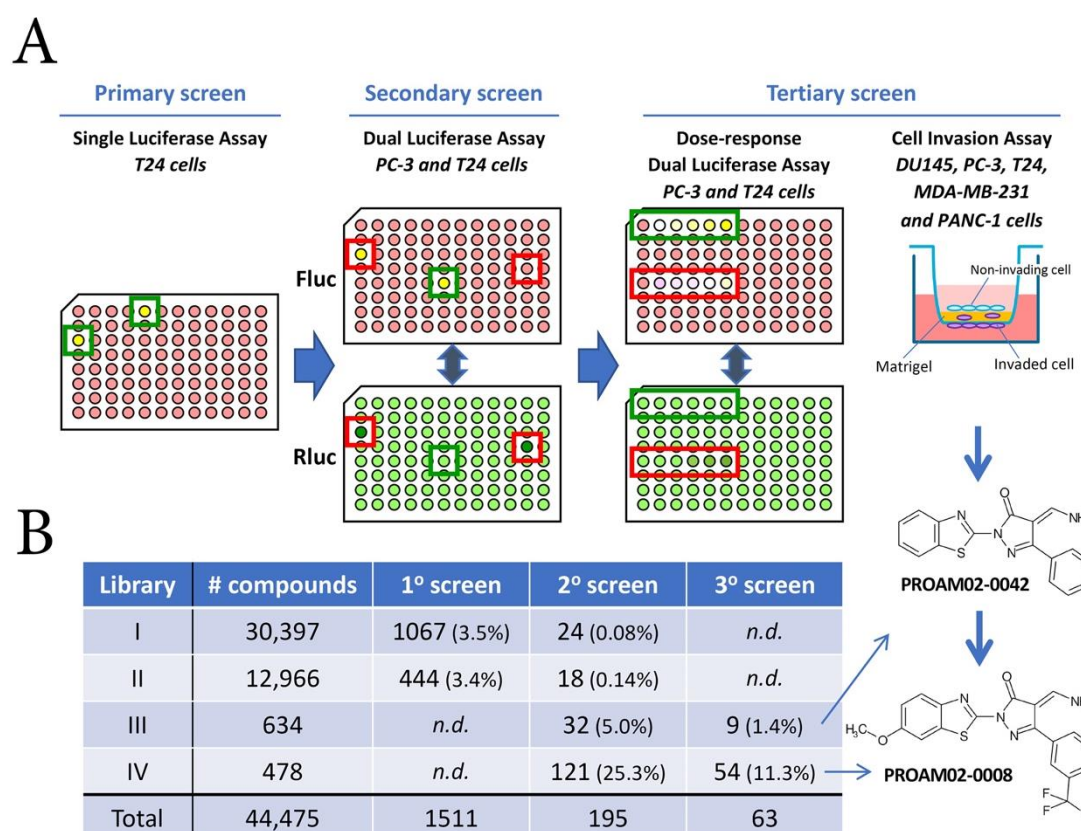
Figure 1. Overview of the screening strategy for the identification of candidate low molecular weight (LMW) compounds ( A ) Three screening rounds were performed with four compound libraries. Initially, libraries I and II were tested in E-cadherin-negative human bladder cancer T24 cells that express the Ecad-Fluc/Rluc reporter construct. In the secondary screen, a dual luciferase assay was performed in PC-3 (E-cadherin intermediate-positive) and T24 (E-cadherin-negative) cells that express the Ecad-Fluc/Rluc reporter construct. Compounds identified in the primary screening round and compounds from libraries III and IV were used. During the third round of screening, dose-response dual luciferase assays were performed in both reporter models. In addition, invasion assays were performed in multiple human cancer cell lines, including DU145, PC-3, T24, MDA-MB-231 and Panc-1 cells. Firefly luciferase-positive wells are indicated in yellow, and Renilla luciferase-positive wells are depicted in green. Excluded wells are depicted in red boxes due to aberrant Renilla luciferase values. ( B ) Overview of the number of compounds tested and identified in the three screening rounds. N.D. = not determined.
