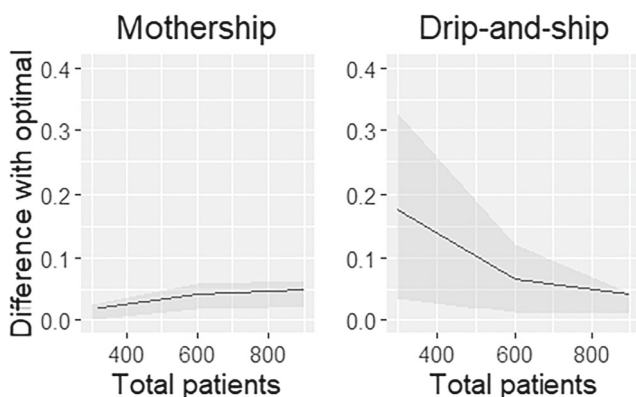
Fig. 9 Mean relative difference with the optimal protocol against P (the area between the 25% and 75% percentile is shaded)
