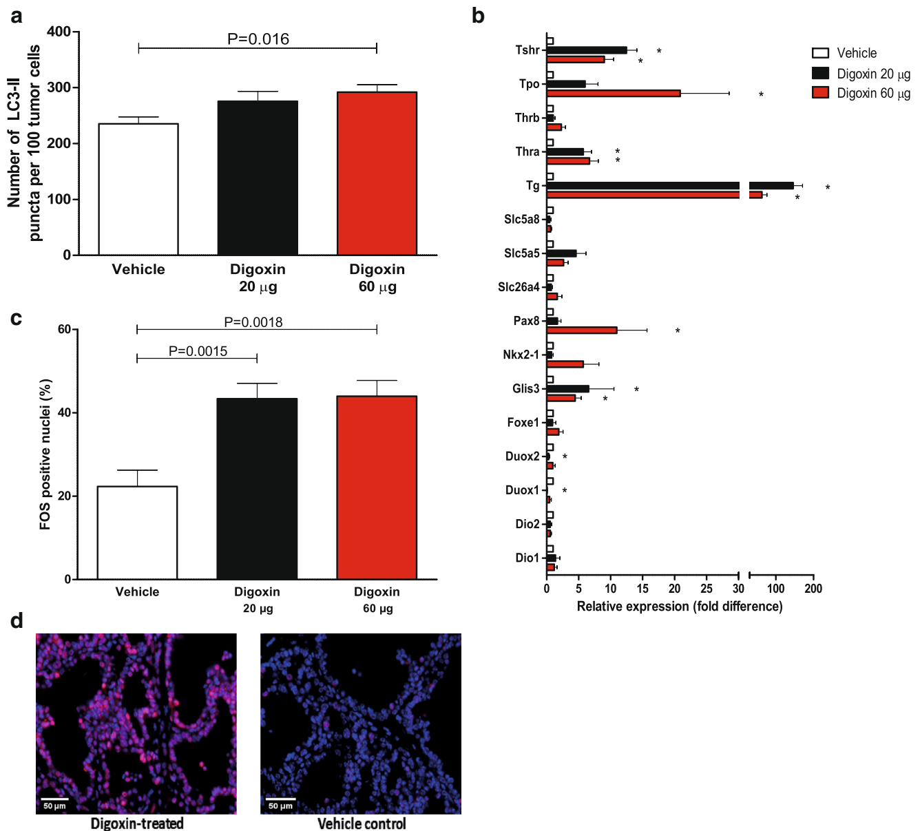
Fig. 3 Digoxin treatment enhances autophagy activity, thyroid-specific gene expression and nuclear FOS levels in Braf V600E mouse tumors. a Quantification of the number of LC3-II positive puncta per 100 tumor cells in post-mortem tumor tissue of TPO-Cre/LSL- Braf V600E transgenic mice treated with either DMSO vehicle (N = 3), 20 µg digoxin (N = 6) or 60 µg digoxin daily (N = 6). Scoring results were generated in quintuple for each tissue section. Data are means ± SEM, * P < 0.05 (Mann-Whitney U test). b Expression of 16 thyroid-specific genes, encompassing the Thyroid Differentiation Score (TDS), in post-mortem tumor tissue of TPO-Cre/LSL- Braf V600E transgenic mice treated with
