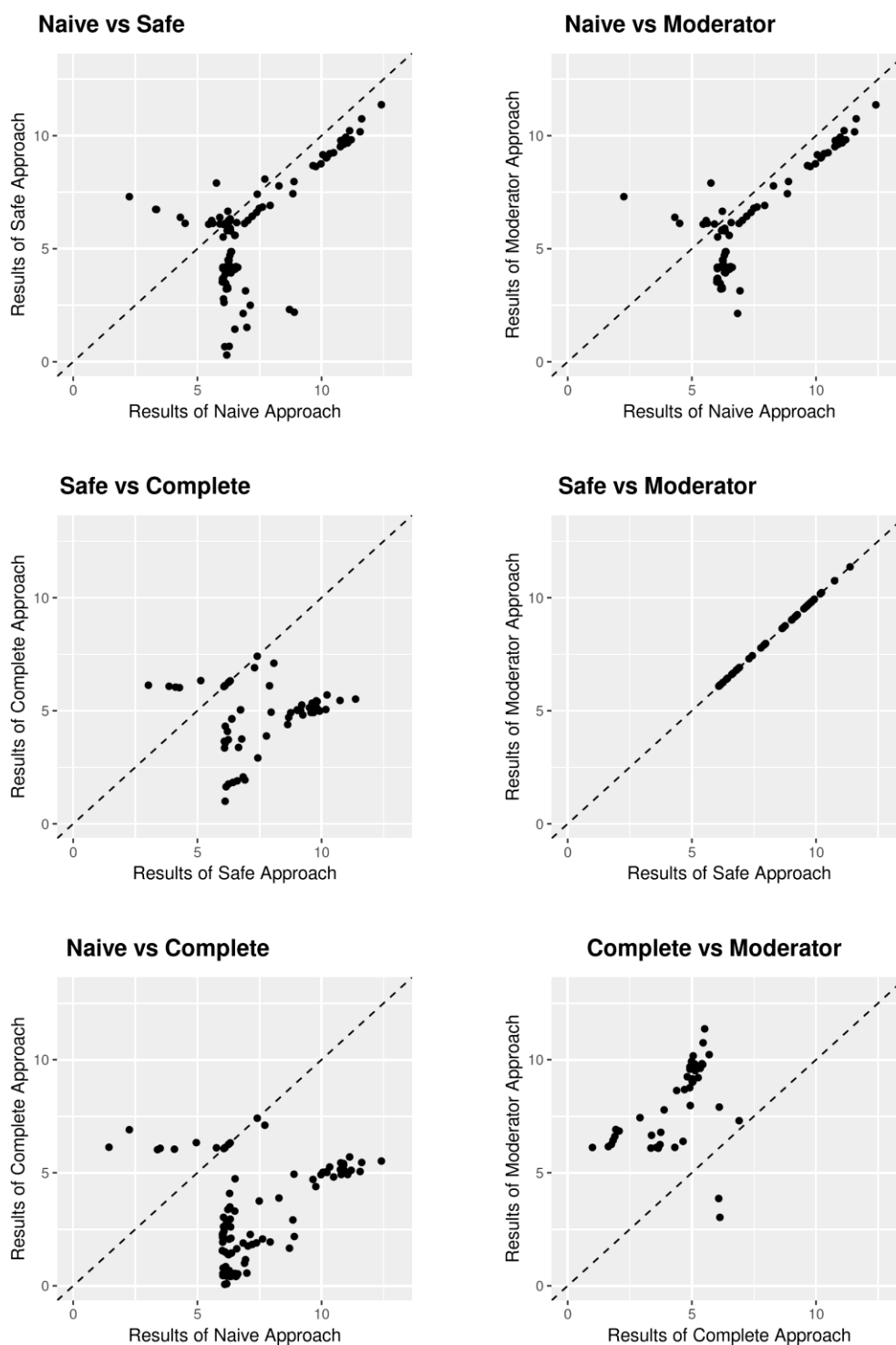
Figure 3. Scatterplots of comparison between four approaches in terms of -\log_{10} (p-value). Each plot shows SNPs with p-value < 10^{-6} for any of the two approaches being compared in the plot.
