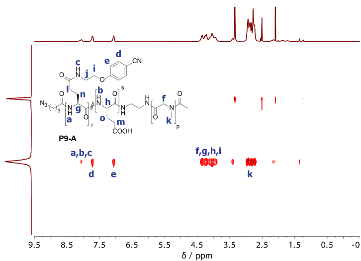
Figure S33. DOSY NMR spectrum of P9-A (pSar 140 -b-pGlu(Mod) 20 ) in DMSO- d 6 .
