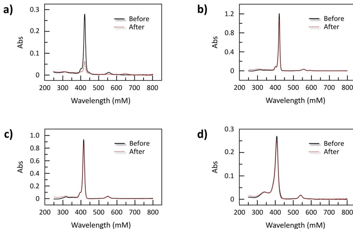
Figure AII.13 Absorption spectra of 2 \mu\text{M} a) [\text{Zn-OMeP}]^{4-} , b) [\text{Zn-MeP}]^{4-} , c) [\text{Zn-F8P}]^{4-} , and d) [\text{Zn-F16P}]^{4-} before (black solid) and after (red short dot) 48 hours irradiation (LED lamp, 450 nm, 16 mW) in 0.1 M sodium phosphate buffer (pH 7.0) under air, T = 298\text{ K} .
