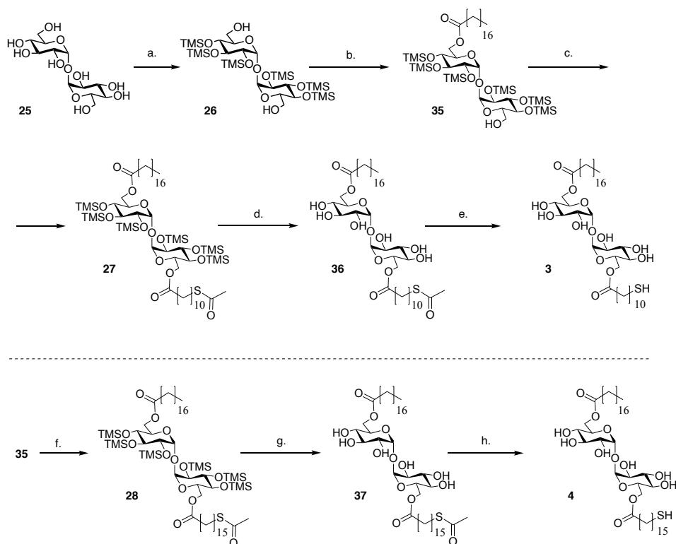
S4 Figure - Synthetic scheme for the generation of trehalose dimycolate analogues. a) i. N,O-bis(trimethylsilyl)acetamide, TBAF, DMF, ii. K 2 CO 3 , MeOH, y: 79%, b) stearic acid, EDCI, DMAP, toluene, y: 47%, c) 11-(acetylthio)undecanoic acid, EDCI, DMAP, toluene, y: 70%, d) amberlite H + , DCM/MeOH 1:1, y: quant., e) NH 2 NH 2 CH 2 COOH, DCM/MeOH 1:1, y: quant., f) 11-(acetylthio)hexadecanoic acid, EDCI, DMAP, toluene, y: 85%, g) amberlite H + , DCM/MeOH 1:1, y: 87%, h) NH 2 NH 2 H 2 O, DCM/MeOH 1:1, y: quant. (isolated as mixture of oxidized and reduced thiol).
