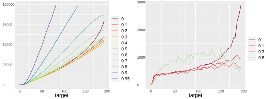
Figure 4.10: Left: Average fixed-target running times of the (50 + 50) GA with uniform crossover and standard bit mutation on LEADINGONES in 200 dimensions, for different crossover probabilities p_c . Results are averages of 100 independent runs. Right: Gradient of selected fixed-target curves.
