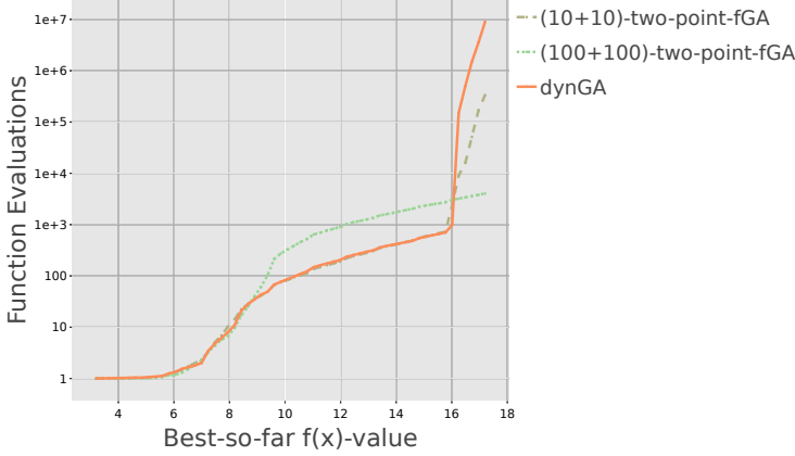
Figure 7.4: Fixed-target ERTs of GAs on F24 in dimension d = 100 . The dynGA switches from the (10 + 10) -two-point-fGA to the (100 + 100) -two-point-fGA at the target f(x) = 15.81 . Results are from 100 independent runs.
