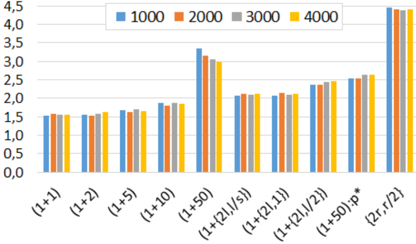
Figure 4.1: Average optimization times for 100 independent runs of the (1 + \lambda) \text{EA}_{>0} variants for ONEMAX, normalized by n \ln n . (Initial) population size for the adaptive variants is 50. p^* = \ln(\lambda)/(2n)
