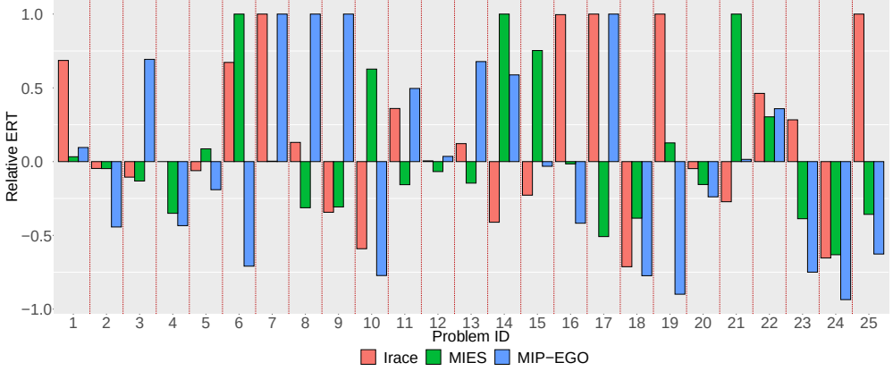
Figure 6.1: Relative ERT values of the GAs obtained by Irace, MIES, and MIP-EGO using ERT as the cost metric compared to the ERT of the GAs obtained by the same method when using AUC as the cost metric during the configuration process. Plotted values are (\text{ERT}_{\text{using ERT}} - \text{ERT}_{\text{using AUC}}) / \text{ERT}_{\text{using AUC}} , capped at -1 and 1 . Positive values therefore indicate that configurator obtains better results when configuring AUC.
