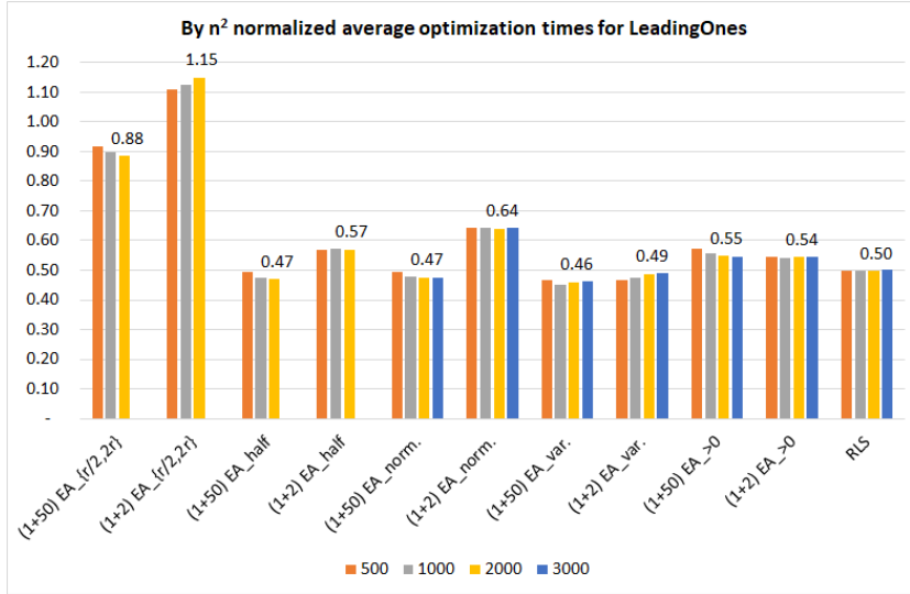
Figure 4.8: By n^2 normalized average optimization times for LEADINGONES, for n between 500 and 3,000. Displayed numbers are for n = 2,000 .
