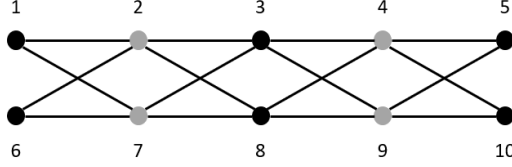
Figure 2.5: A scalable maximum independent set problem, with n = 10 vertices and the optimal solution of size 6 marked by the black vertices.
