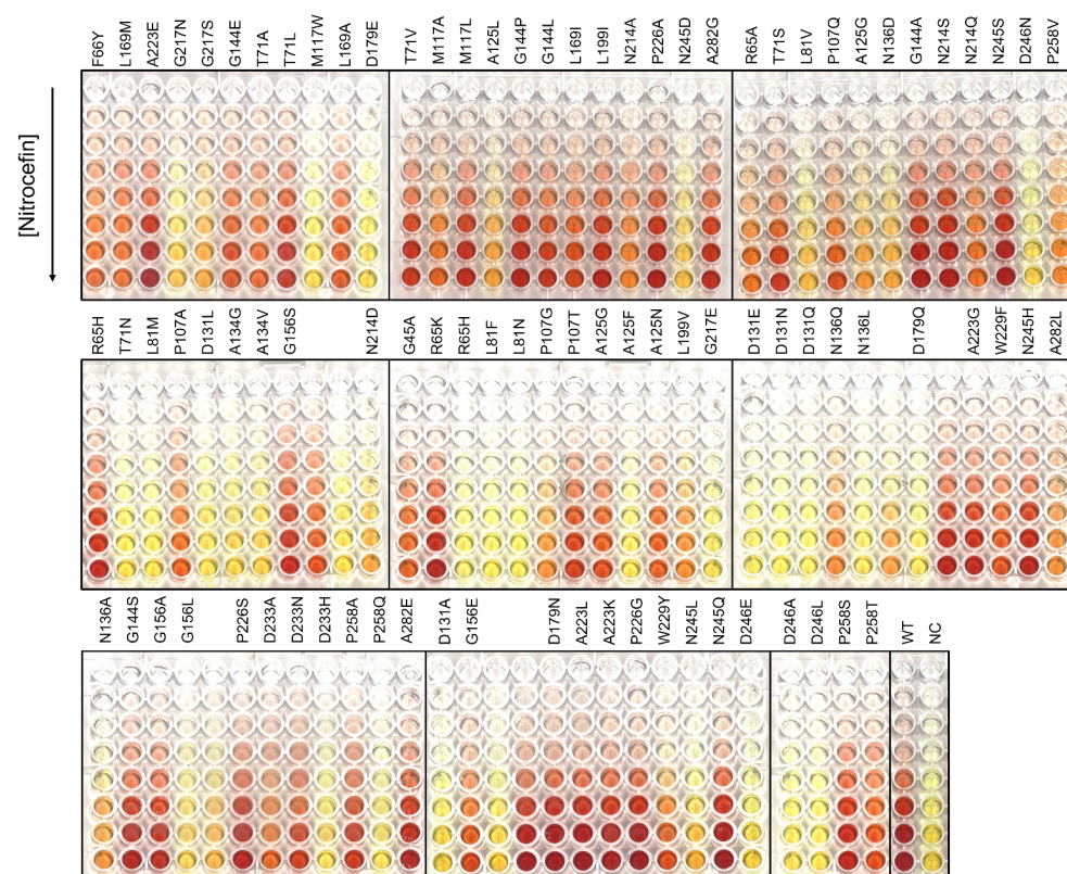
Figure S2.3. Plates with the range of nitrocefirin concentration and whole lysates containing BlaC variants after 5 minutes of reaction. Non-labeled wells contain mutants of residues with lower percent conservation, thus not discussed within this study.
