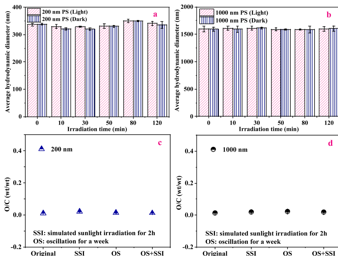
Figure 2. Average hydrodynamic diameters of PS (20 mg/L) during simulated sunlight irradiation after 1 week of oscillation (a, b) and the O/C ratio (wt/wt) of PS after treatment with oscillation and light irradiation (c, d). Oscillation conditions: 150 rpm, 25 °C.
