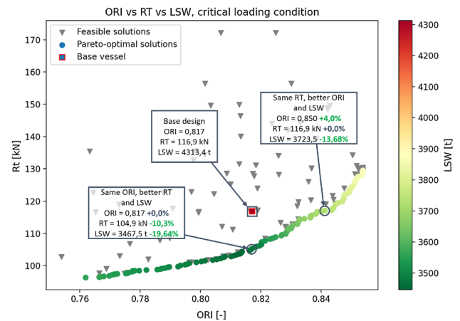
Fig. 5 Pareto Frontier of Ship Design case with Original Design by human expert represented by a square. Objectives are maximize the Operability Robustness Index (ORI[-]), minimize ship resistance ( R_t [kN]), and minimize Lightship Weight (LSW[t])
