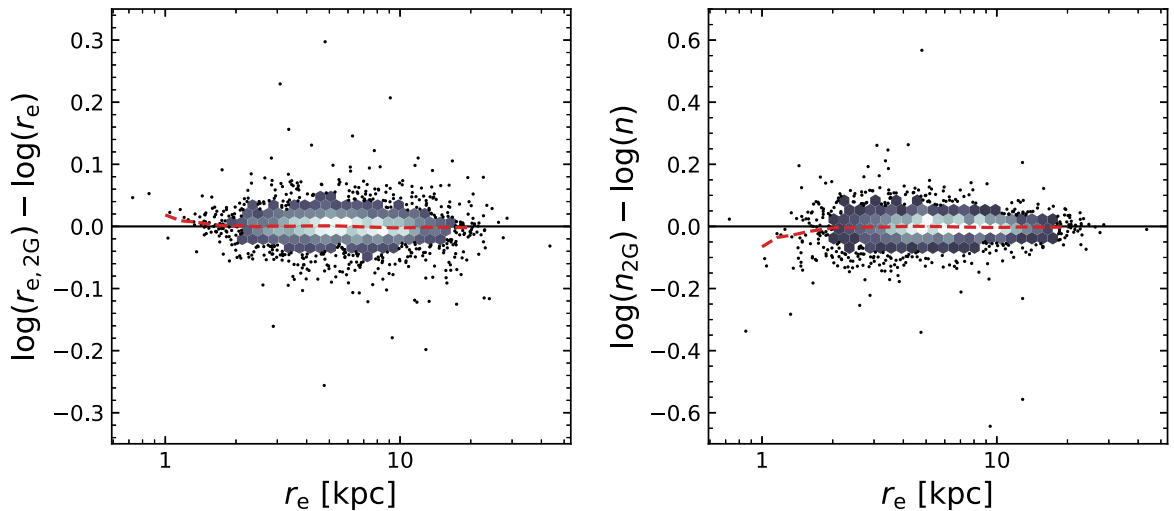
Figure B2. The difference in the inferred r -band size (left) and Sérsic index (right) between the images that are convolved with a single Gaussian PSF and a double Gaussian PSF. There is no systematic offset between the two sets of models (medians are indicated with a red, dashed line), and the scatter is consistent with the random uncertainties discussed in Section 3.2.4. Only for very small galaxies ( r_e \lesssim 2 kpc), where we may expect to see the largest impact of a difference in the PSF, does there appear to be a slight offset in both the size and Sérsic index, of up to \Delta \log(r_e) \sim 0.05 dex and \Delta \log(n) \sim -0.1 dex. The choice of adopting a simple (single Gaussian) PSF shape thus has minimal impact on the results presented in this work.
