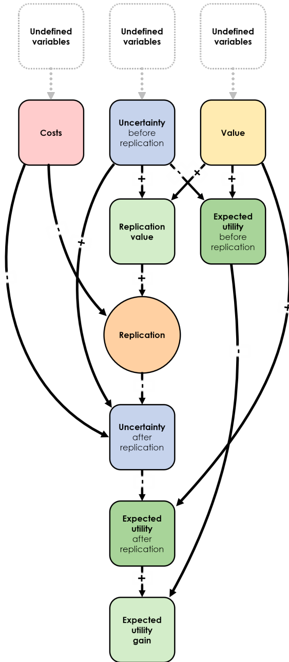
Figure 1: Structural causal model of the system that determines replication value. Arrow direction signals the causal direction of effects. Time flows from the top to the bottom of the figure; variables (nodes) closer to the top are determined earlier in time than nodes closer to the bottom (e.g., the value of “Costs” is determined before the value of “Replication”). The “+” and “-” signs on the arrows indicate whether the effect is positive or negative. Consult Table 1 for variable definitions and the structural equations that determine the value of each variable in the graph.
