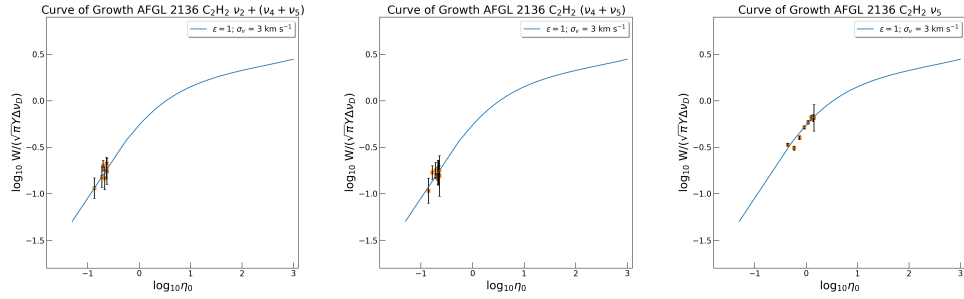
Figure 5.17: Curves of growth for the \nu_2 + (\nu_4 + \nu_5) ( 3\ \mu\text{m} ), (\nu_4 + \nu_5) ( 7\ \mu\text{m} ) and \nu_5 ( 13\ \mu\text{m} ) bands of \text{C}_2\text{H}_2 in AFGL 2136, calculated for the disk model. Equivalent widths for the (\nu_4 + \nu_5) and \nu_5 bands are taken from chapter 3. Curves of growth are constructed for a \sigma_v = 3\ \text{km s}^{-1} and \epsilon = 1 .
