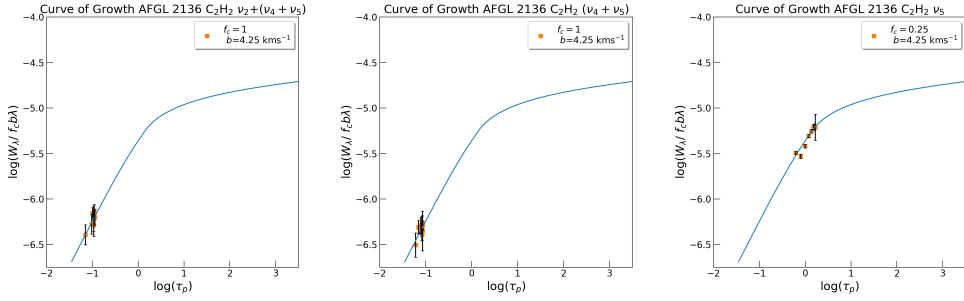
Figure 5.16: Curves of growth for the \nu_2 + (\nu_4 + \nu_5) ( 3\ \mu\text{m} ), (\nu_4 + \nu_5) ( 7\ \mu\text{m} ) and \nu_5 ( 13\ \mu\text{m} ) bands of \text{C}_2\text{H}_2 in AFGL 2136, calculated using the absorbing foreground slab model. Equivalent widths for the (\nu_4 + \nu_5) and \nu_5 bands are taken from chapter 3. A covering factor of 1 is used for the 3\ \mu\text{m} and 7\ \mu\text{m} lines, and 0.25 for the 13\ \mu\text{m} lines. A Doppler parameter of 4.25\ \text{km s}^{-1} is considered, consistent with the disk model ( \sigma_v = 3\ \text{km s}^{-1} ).
