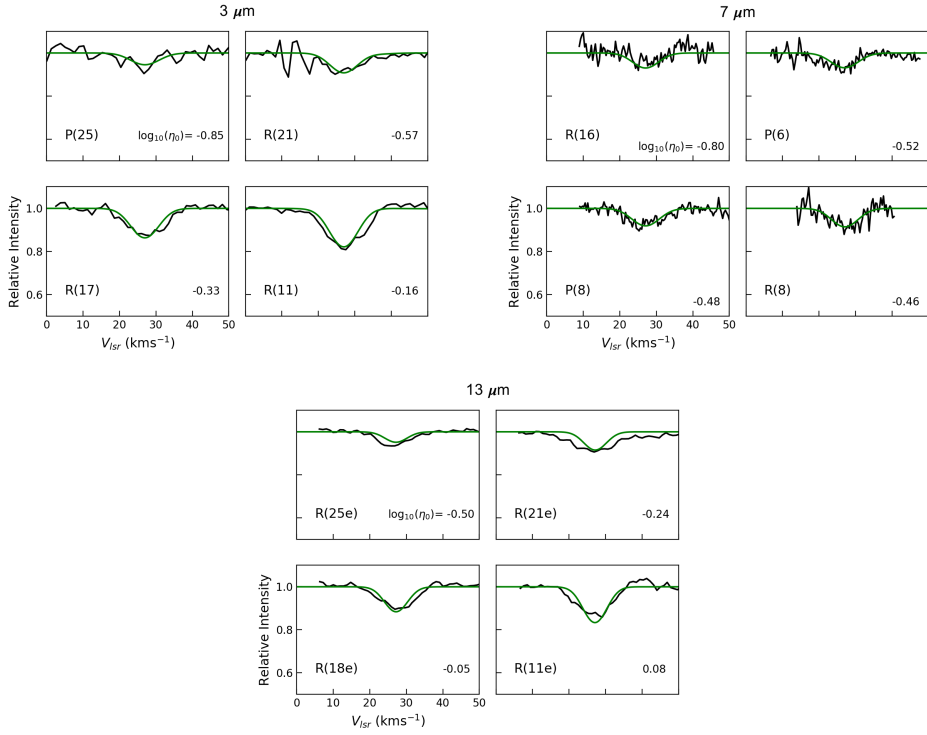
Figure 5.11: Absorption lines of varying opacity from the \nu_1 (3 \mu\text{m} ), \nu_2 v_2=2-0 (7 \mu\text{m} ) and \nu_2 (13 \mu\text{m} ) bands of HCN (top left, top right and bottom respectively). The green solid line denotes a model of a background light source seen through a dust-free absorbing slab of gas, generated at the physical conditions derived from the curve of growth of the \nu_1 band. The opacities of each line derived from the disk model curve of growth, \eta_0 , are indicated in the corresponding panels. A covering factor of 1 is used for the 3 \mu\text{m} and 7 \mu\text{m} lines, and a covering factor of 0.3 is used for the 13 \mu\text{m} lines.
