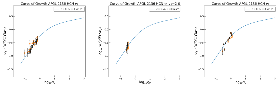
Figure 5.13: Curves of growth for the \nu_1 ( 3\ \mu\text{m} ), \nu_2 = 2-0 ( 7\ \mu\text{m} ) and \nu_2 ( 13\ \mu\text{m} ) bands of HCN in AFGL 2136, calculated for the disk model. Equivalent widths for the \nu_2 and \nu_2\ v_2=2-0 bands are taken from chapter 3. Curves of growth are constructed for a \sigma_v = 3\ \text{km s}^{-1} and \epsilon = 1 .
