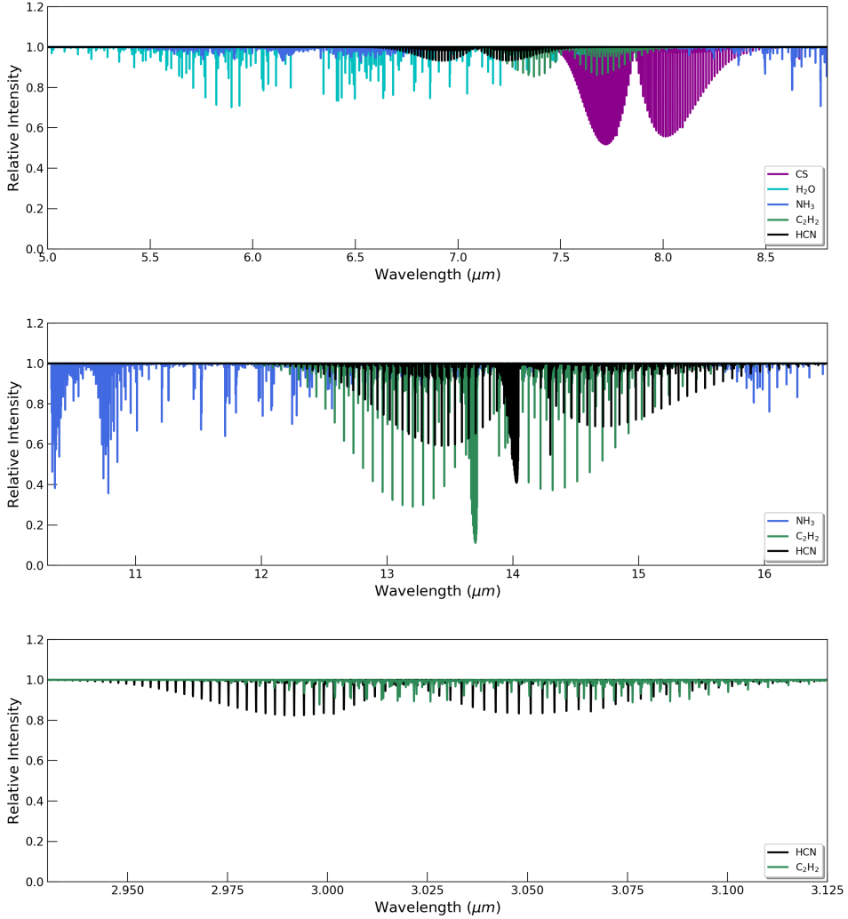
Figure 1.6: Model absorption line spectra of \text{H}_2\text{O} , \text{HCN} , \text{C}_2\text{H}_2 , \text{NH}_3 and \text{CS} at a column density of 1 \times 10^{17} \text{ cm}^{-2} and a temperature of 500 K. The \text{H}_2\text{O} lines are relatively weak compared to the other species, however in practice, these lines are observed to be the strongest due to the large column density in star forming regions ( 10^{18} \text{ cm}^{-2} ). The bands at 13 \mu\text{m} are stronger relative to the bands at other wavelengths for \text{HCN} , \text{C}_2\text{H}_2 and \text{NH}_3 .
