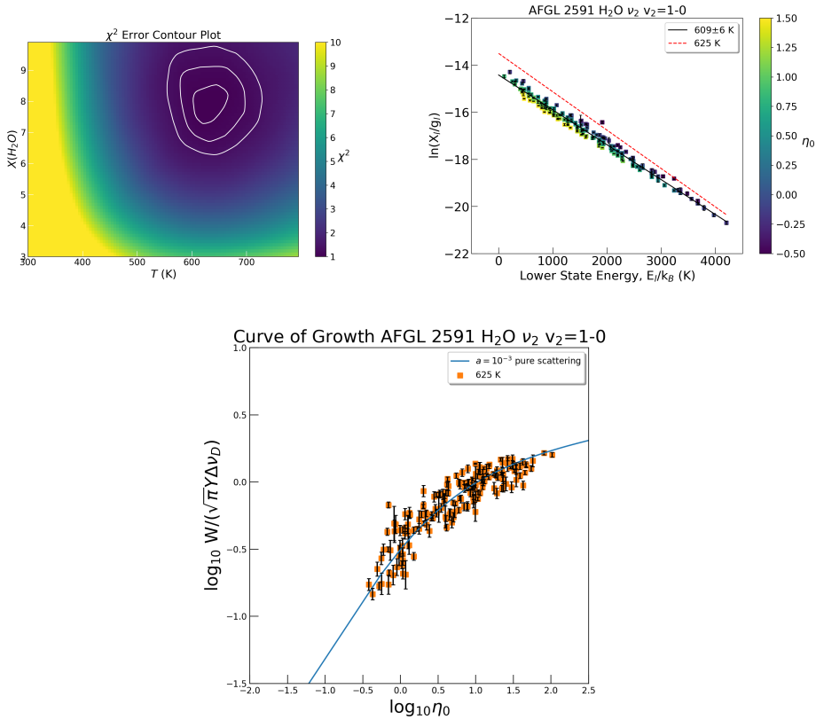
Figure 4.18: bottom : The curve of growth for the v=1-0 transition of AFGL 2591. The theoretical curve is for the case of \epsilon = 0 . The empirical curve of growth is calculated based on the physical conditions given in Table 4.2. top left : The error on the parameters is given in the contour plot where the colour scale is the reduced \chi^2 value. The contours represent the 1\sigma , 2\sigma and 3\sigma uncertainty levels. The H 2 O abundance is quoted relative to CO. top right : The rotation diagram is a function of \eta_0 and the abundances for the optically thick lines were determined using the curve of growth. The best fit temperature of 625 K from the curve of growth is represented by the red dashed line. The black solid line is a fit to the corrected data set and the corresponding temperature is indicated. Note that the y-axis is the abundance in the lower level based on the stellar atmosphere theory.
