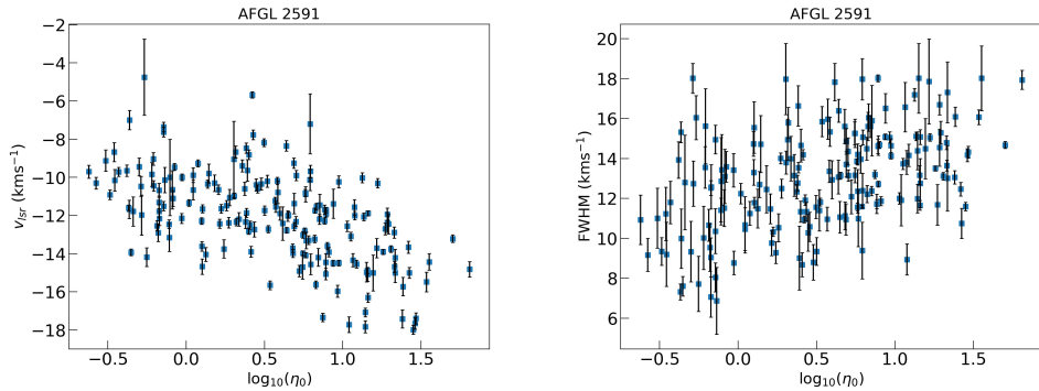
Figure 4.13: Plots illustrating the relationship between \eta_0 and the peak velocity and line width in AFGL 2591 on the left and right, respectively.
