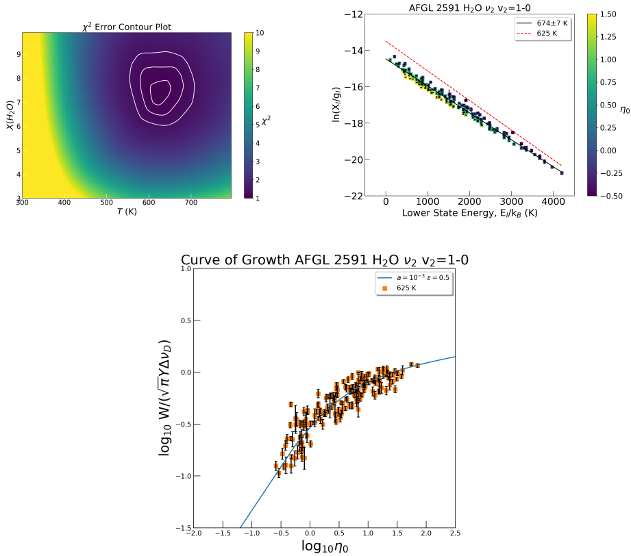
Figure 4.17: bottom : The curve of growth for the v=1-0 transition of AFGL 2591. The theoretical curve is for the case of \epsilon = 0.5 . The empirical curve of growth is calculated based on the physical conditions given in Table 4.2. top left : The error on the parameters is given in the contour plot where the colour scale is the reduced \chi^2 value. The contours represent the 1\sigma , 2\sigma and 3\sigma uncertainty levels. The \text{H}_2\text{O} abundance is quoted relative to CO. top right : The rotation diagram is a function of \eta_0 and the abundances for the optically thick lines were determined using the curve of growth. The best fit temperature of 625 K from the curve of growth is represented by the red dashed line. The black solid line is a fit to the corrected data set and the corresponding temperature is indicated. Note that the y-axis is the abundance in the lower level based on the stellar atmosphere theory.
