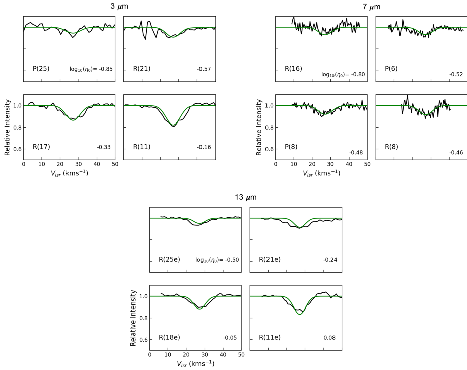
Figure 5.11: Absorption lines of varying opacity from the \nu_1 ( 3 \mu\text{m} ), \nu_2 v_2=2-0 ( 7 \mu\text{m} ) and \nu_2 ( 13 \mu\text{m} ) bands of HCN (top left, top right and bottom respectively). The green solid line denotes a model of a background light source seen through a dust-free absorbing slab of gas, generated at the physical conditions derived from the curve of growth of the \nu_1 band. The opacities of each line derived from the disk model curve of growth, \eta_0 , are indicated in the corresponding panels. A covering factor of 1 is used for the 3 \mu\text{m} and 7 \mu\text{m} lines, and a covering factor of 0.3 is used for the 13 \mu\text{m} lines.
