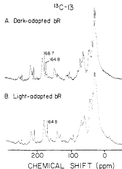
FIGURE 4: 13 C MAS spectra of 13 C-13 bR in the dark-adapted (A) and light-adapted (B) states.
