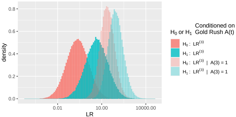
Figure 5.5. Sampling distributions under the null ( H_0 ) and alternative ( H_1 ) hypothesis of likelihood ratios LR^{(3)} = \prod_{i=1}^3 \phi_0(Z_i)/\phi_0(Z_i) of three studies with and without extreme Gold Rush accumulation bias A(t) . Note that the x-axis is on a log scale.
