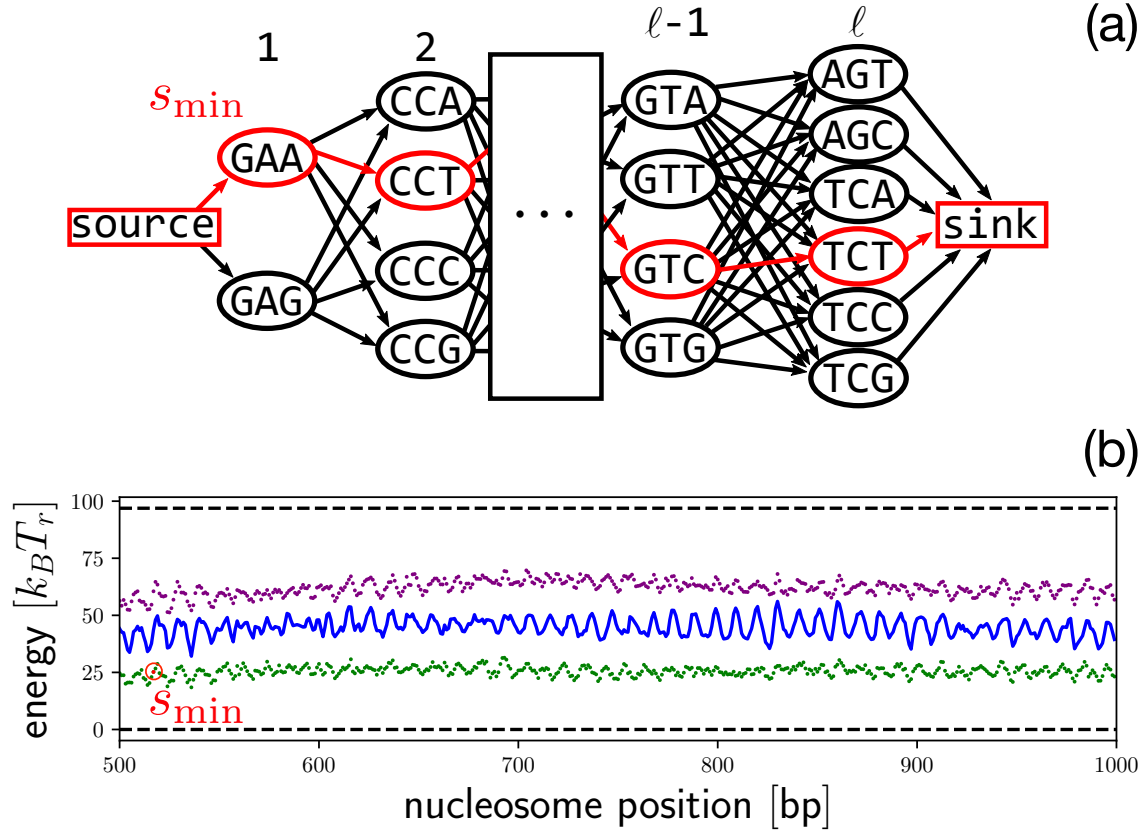
Figure 3.5: (a) Graph \mathcal{G}_{\text{gene}} shows all synonymous ways to encode for a given amino acid sequence ( \ell is either 49 or 50). The shortest energy path s_{\text{min}} is highlighted. (b) Energy landscape of a 500 bp stretch of gene YAL002W from yeast (solid curve), pointwise minimal and maximal energies through synonymous mutations (dotted curves) and total minimum and maximum (dashed lines). s_{\text{min}} is the same sequence as in (a).
