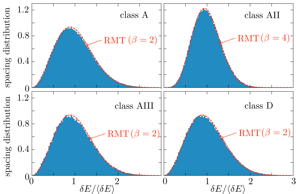
Figure 2: Histograms: Spacing distributions computed from the discretized Dirac Hamiltonian (5.1), with different types of disorder corresponding to the four symmetry classes in Table 1. The red dashed line is the prediction (5.2) from random-matrix theory in the presence of symplectic symmetry ( \beta = 4 ) and in its absence ( \beta = 2 ).
