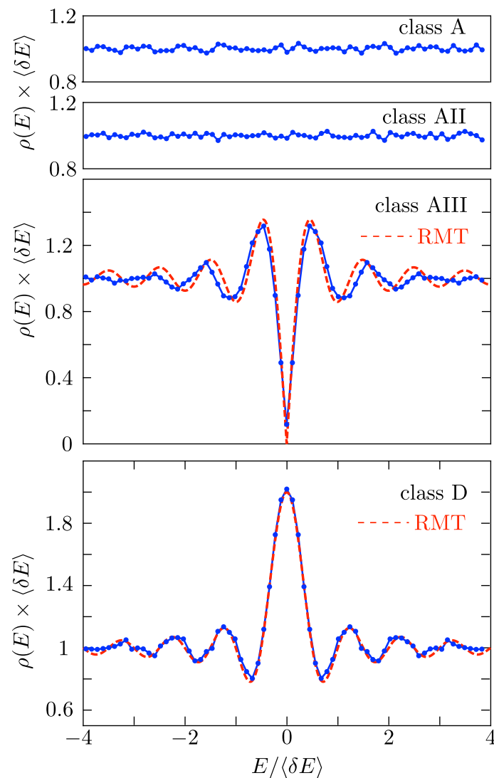
Figure 3: Density of states in the four symmetry classes, calculated numerically from the discretized Dirac Hamiltonian (blue solid lines) and compared with the RMT prediction (5.3) (red dashed lines). Chiral symmetry introduces a linear dip (class AIII), while particle-hole symmetry introduces a quadratic peak (class D).
