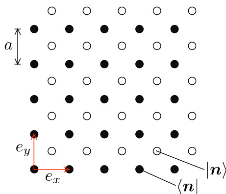
Figure 1: A pair of staggered grids (lattice constant a , lattice vectors e_x, e_y ) used in the Stacey discretization of the 2D Dirac equation. The wave function and its spatial derivatives are evaluated at the open lattice points, in terms of the values on the four neighboring closed lattice points. The basis states \langle \mathbf{n} | and |\mathbf{n}\rangle on the two lattices are indicated.
