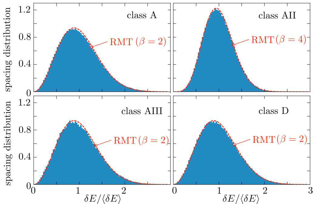
Figure 2: Histograms: Spacing distributions computed from the discretized Dirac Hamiltonian (5.1), with different types of disorder corresponding to the four symmetry classes in Table 1. The red dashed line is the prediction (5.2) from random-matrix theory in the presence of symplectic symmetry ( \beta = 4 ) and in its absence ( \beta = 2 ).
