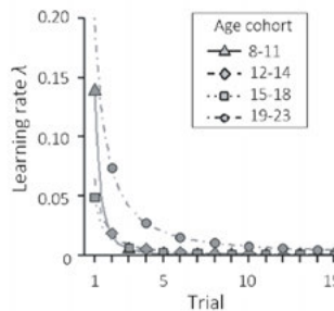
Figure S5. Estimated learning rates per age cohort from the best models for the Non-Social learning task. Best models include decaying learning rates. Estimates learning rates as a function of the trial number, for each of the four age cohorts separately for the Non-Social learning task.
