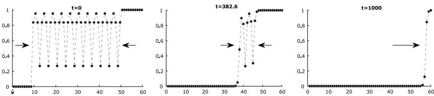
Fig. 4 This sequence of snapshots from a simulation of the Nagumo LDE (21) with a = 0.63 and d = 0.0625 features a collision between a wave of type o \rightarrow o111 and a counterpropagating wave of type o111 \rightarrow 1 . The right part of the intermediate buffer zone is first pulled towards one by the incoming wave on the right, but then gets pulled towards zero by the final travelling monochromatic wave
