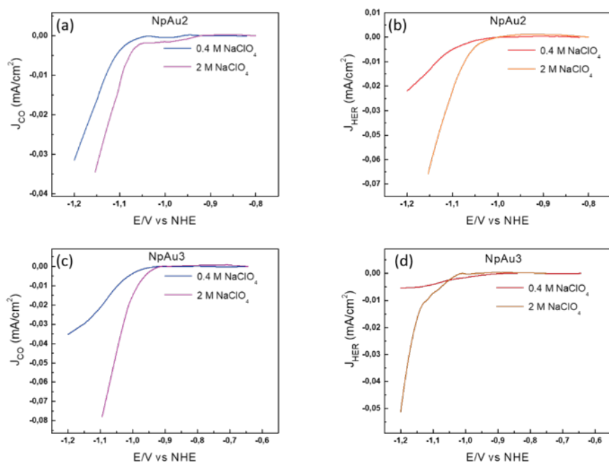
Figure S7 Partial specific current density for CO formation as obtained from the ionic current at m/z 28 by using eqn. 3 (Main Manuscript) with 0.5 atm. CO 2 in 0.1 M NaHCO 3 and 0.4 M NaClO 4 containing electrolyte (blue) and in 0.1 M NaHCO 3 and 2 M NaClO 4 containing electrolyte (purple) at a scan rate of 5 mVs -1 and a flow rate of 300 \mu Lmin -1 on (a) NpAu2 and (c) NpAu3 and Partial current density for HER as obtained from the ionic current at m/z 2 by using eqn. 3 (Main Manuscript) with 0.5 atm. CO 2 in 0.1 M NaHCO 3 and 0.4 M NaClO 4 containing electrolyte (red) and in 0.1 M NaHCO 3 and 2 M NaClO 4 containing electrolyte (orange) at a scan rate of 5 mVs -1 and a flow rate of 300 \mu Lmin -1 on (b) NpAu2 and (d) NpAu3.
