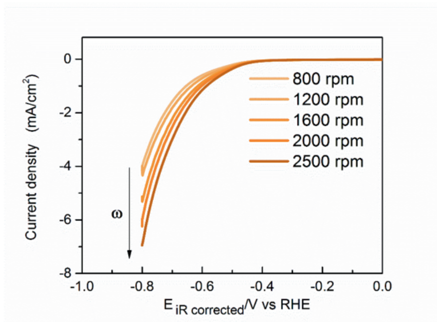
FigureS5 CVs obtained for HER at different rotation rates using the RDE on Au polycrystalline surface in Ar sat. 0.5 M NaHCO 3 at 25 mVs -1 . The direction of the arrow indicates increasing rotation rate.
