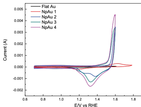
Figure S3 Characterization cyclic voltammograms for different Au catalysts in 0.1 M H_2SO_4 in Ar sat. environment at 50\text{ mVs}^{-1} where the charge of the Au_xO_y reduction peak was used to calculate the electrochemically active surface area (ECSA) of the different samples
