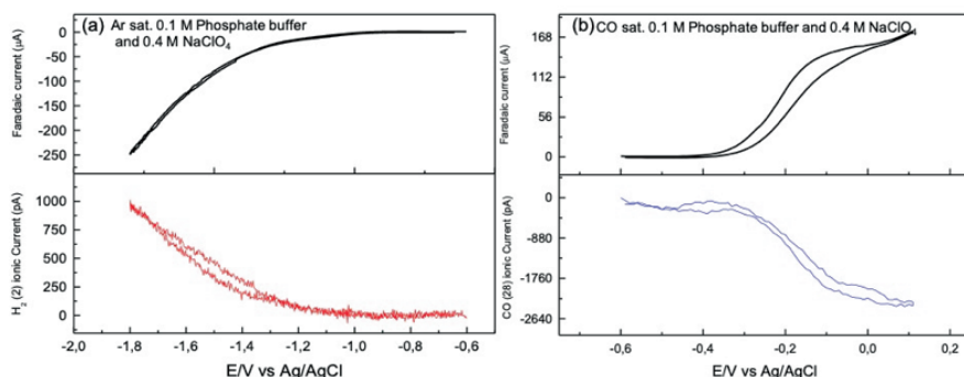
Figure S2 DEMS calibration experiment for (a) H_2 and (b) CO, performed in 0.1 phosphate buffer and 0.4 M NaClO_4 at 5\text{ mVs}^{-1} and a flow rate of 300\text{ }\mu\text{Lmin}^{-1} in Ar sat. and CO sat. conditions respectively. For determining K_{H_2}^a the Faradaic current for HER and the ionic current at m/z 2 as shown in S1a in the top panel and the bottom panel, respectively, were plugged into eqn. 3 (see Section 2.4 in the Main Manuscript) where z was taken to be 2. For determining K_{CO}^a the Faradaic current for CO oxidation and the ionic current at m/z 28 as shown in S1b in the top panel and the bottom panel, respectively, were plugged into eqn. 3 (see Section 2.4 in the Main Manuscript) where z was taken to be 2.
